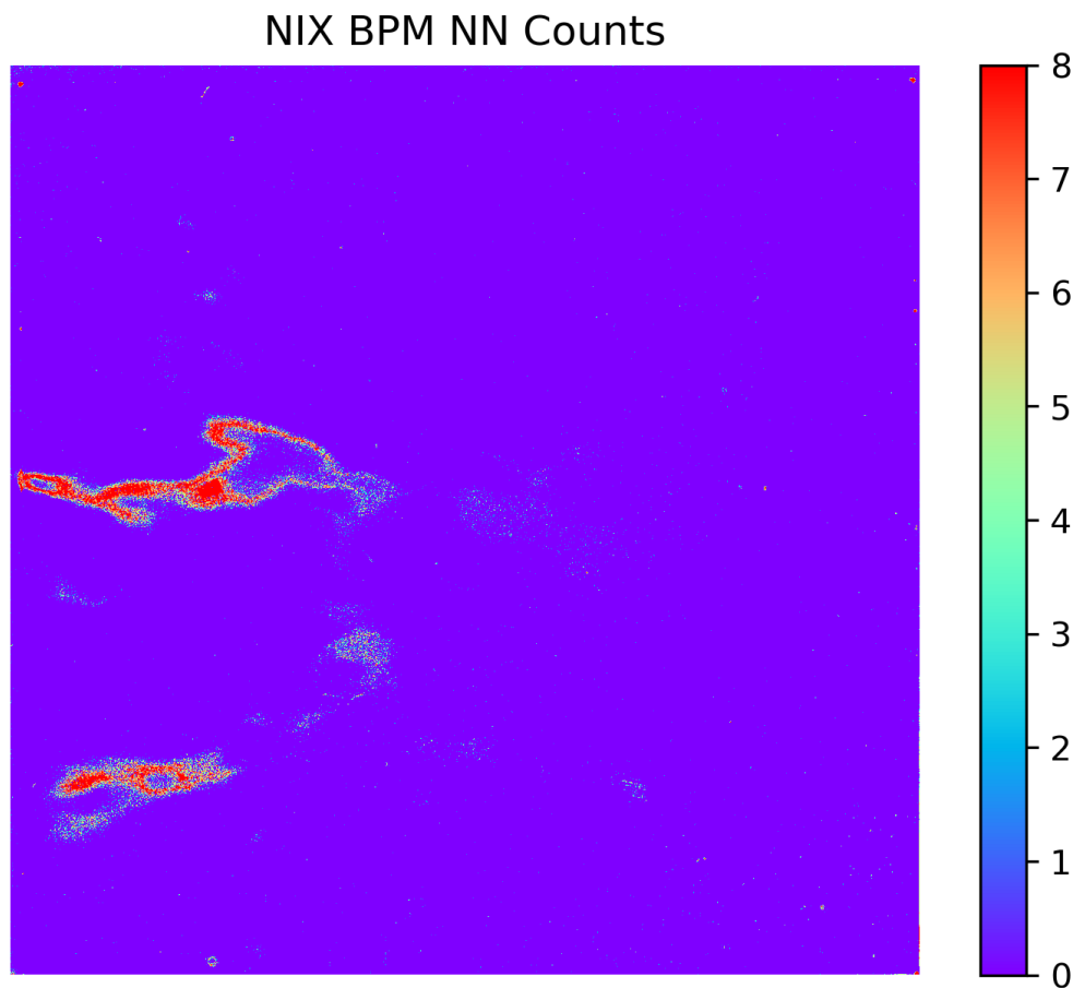
Figure 8: Number of identified bad pixels neighboring each pixel in NIX detector. Pixels which are not identified as bad pixels have a value of 0.
