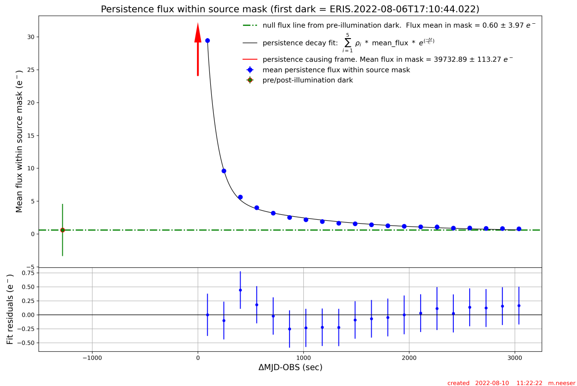
Figure 12: Persistence recovery time of SPIFFIER detector with respect to peak flux.
