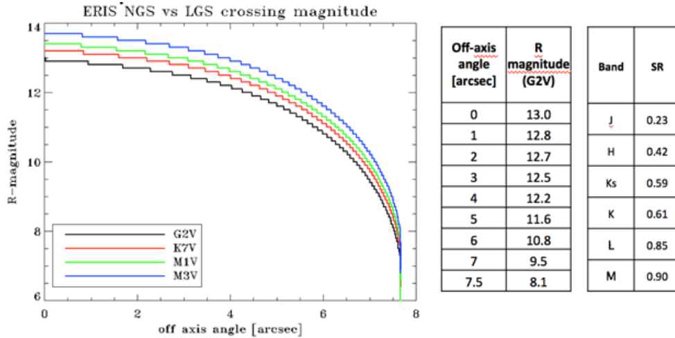
Figure 17: Identification of maximum off axis angle for the NGS WFS reference star for NGS and LGS mode equal performances. The table on the right side shows the limiting magnitude value for equal per-formances and the achieved SR in various bands. The magnitude is given for different star types. The ERIS specifications refer to the G2V type star.
