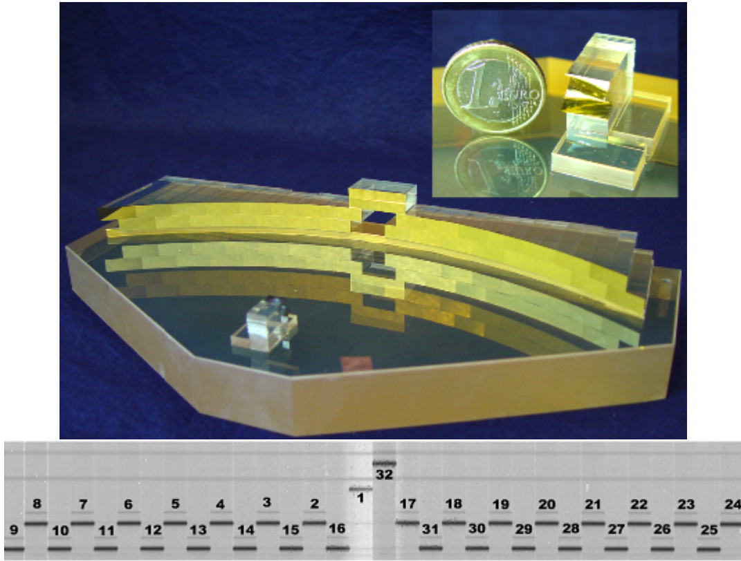
Figure 10: Top: SPIFFIER image slicer (a): The light enters through the hole in the big slicer. A stack of 32 small mirrors, the small slicer (also shown in the sub-panel), slices the image and redirects the light to-wards the 32 mirrors of the big slicer, which re-arranges the slitlets into a 31 cm long pseudo-slit. Bottom: Illustration of the slitlet layout in raw SPIFFIER images, light is dispersed vertically on the science detector.
