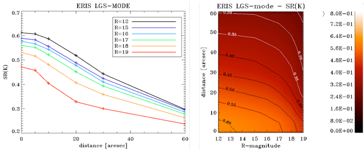
Figure 16: The LGS mode performance as a function of reference star magnitude and off-axis distance from scientific target.
