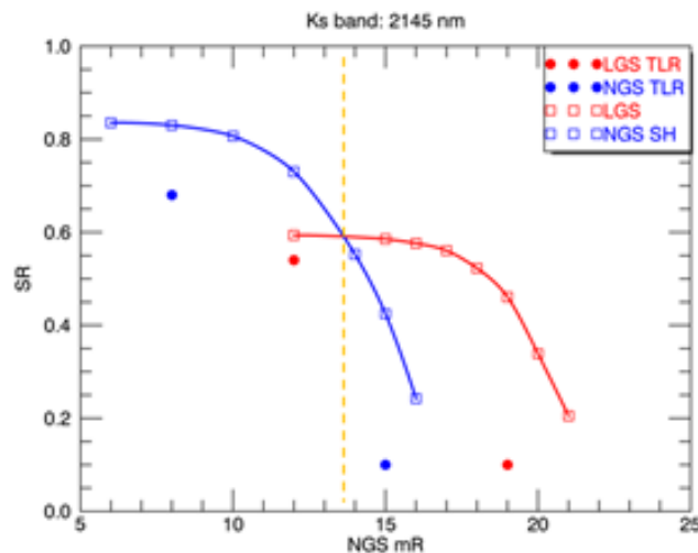
Figure 14: The SR in K band as a function of the reference star magnitude in R band for NGS and LGS case. SR values are given on the y-axis in this plot.
