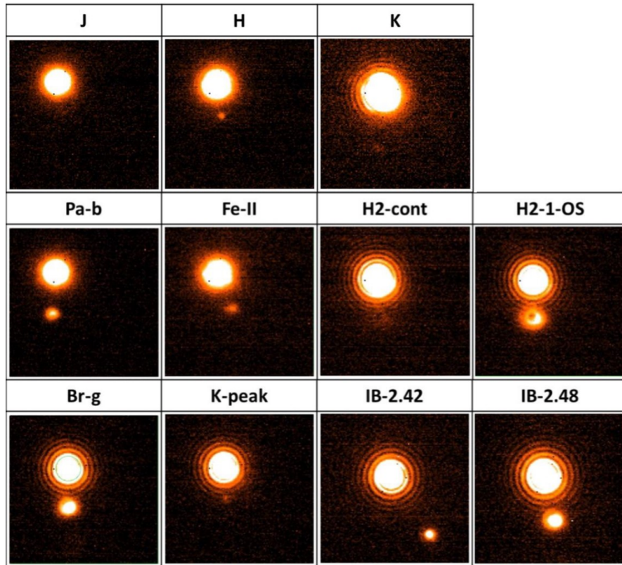
Figure 22: Relative positions and strengths of ghosts in the centre of the field.
