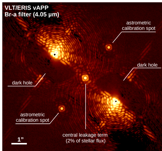
Figure 24: NIX on-sky APP PSF with Br-a filter.
