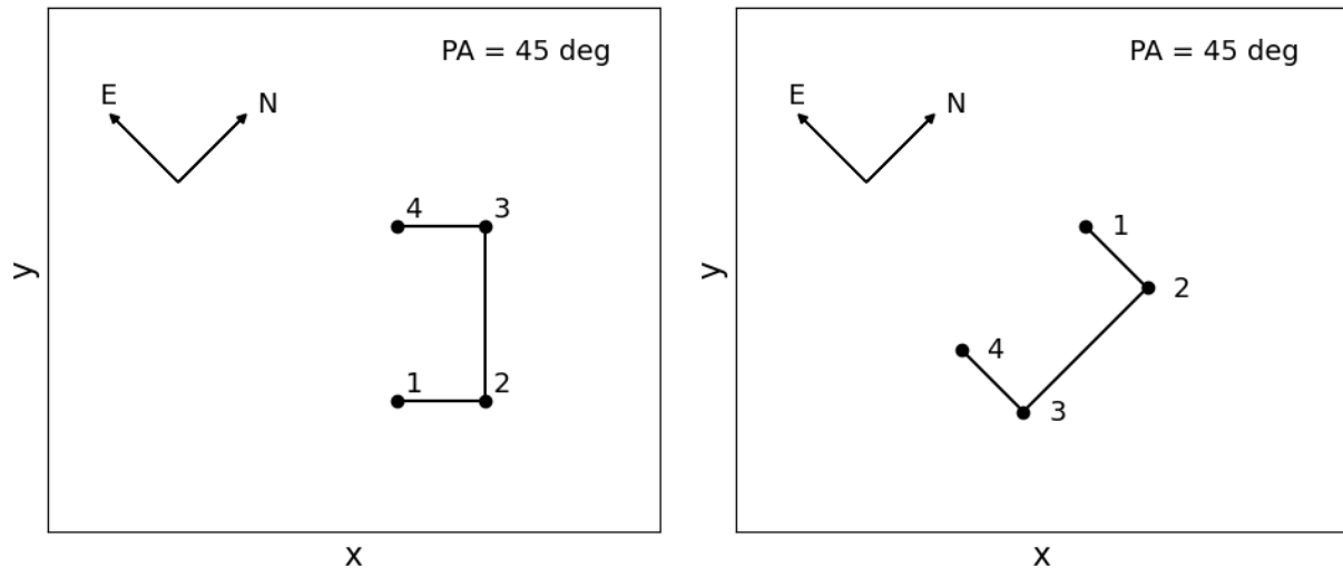
Figure 28: An illustration of the offset sequence for a point source with the on-sky position angle of 45 deg taken with the ERIS_ifs_obs_GenericOffset template. Left side: Offset coordinate type DETECTOR ; Right side: Offset coordinate type SKY . This figure is meant to illustrate where on the detector the image of a point source is showing up, if the telescope is doing the following offset sequence: (0,+1,0,-1) in X or RA and (0,0,+2,0) in Y or DEC. The numbers illustrate the order of the offsets.
