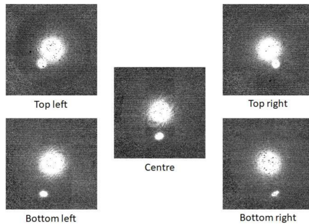
Figure 23: Dependency of relative ghost position on location in field, illustrated with the Pa-b filter.
