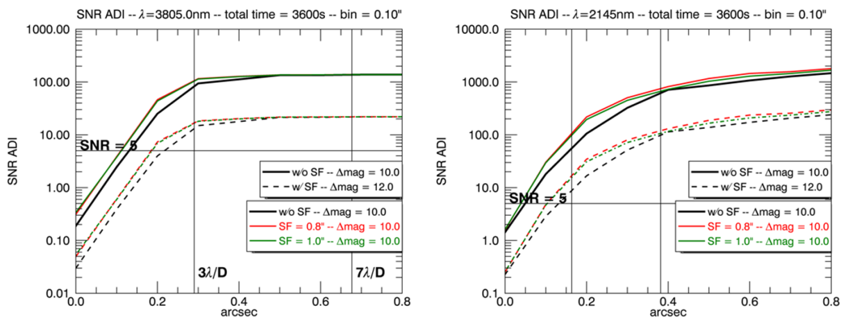
Figure 20: The SNR for L' (left) and K band (right) computed with numerical simulations when AO corrected images are combined by using ADI technique. The SNR saturates quickly in the L' case because of the large contribution from sky background.
