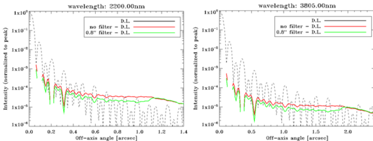
Figure 21: The corrected PSFs profiles at K and L' band for the two options baseline and filtered SH for the NGS WFS. Different behavior is given by red and green line respectively. DL in the figure labels means Diffraction Limit.
