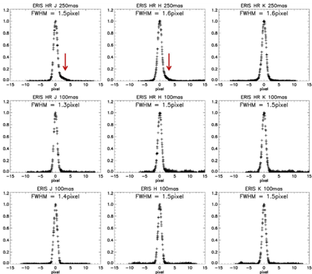
Figure 26: Fine sampled SPIFFIER line profiles at selected pixel scales. Red arrows indicate the asymmetries in line profiles.
