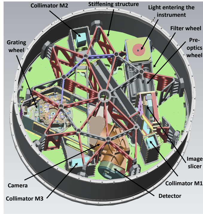
Figure 9: An inside view of the SPIFFIER cryostat with indications for the locations of various opto-mechanical elements. Some housing covers and parts of the stiffening structure are not shown for better illustration. The diameter of the instrument is 1.3m.
