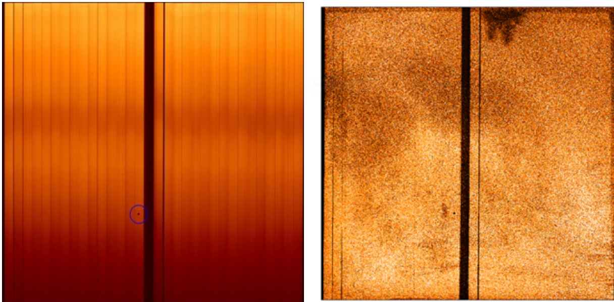
Figure 11: Left: SPIFFIER K.low flat at 25 mas pixel scale. A clump of cold pixels is marked with circle in the left panel. Right: 2D persistence map after a 5-minute long flat exposure.
