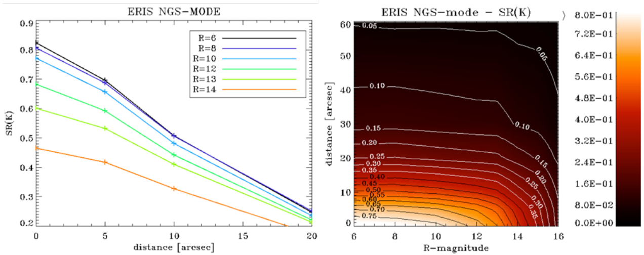
Figure 15: The NGS mode performance as a function of reference star magnitude and off-axis distance from scientific target.
