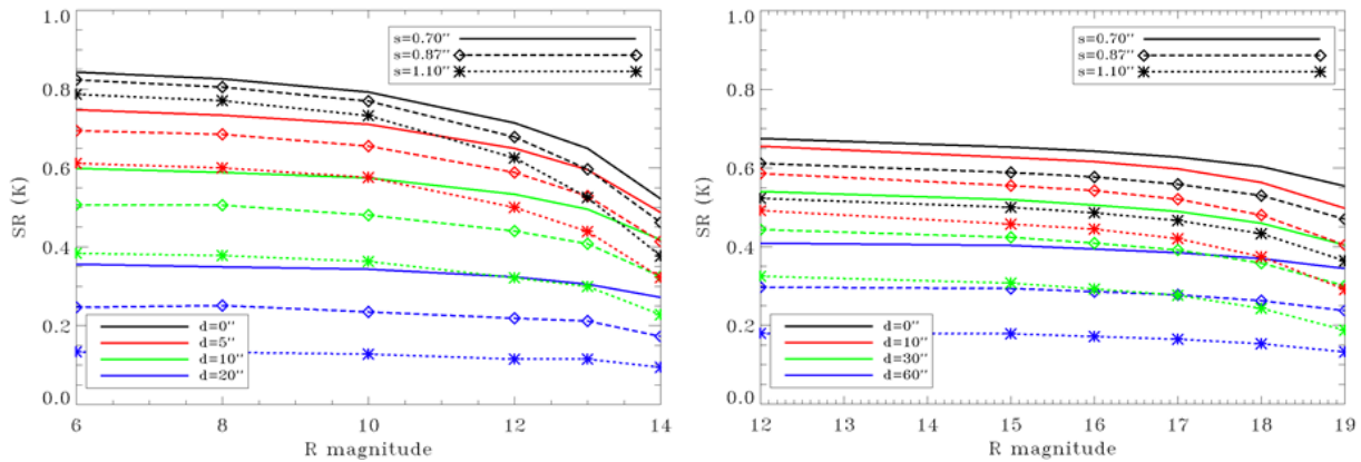
Figure 18: K band SR for 3 different seeing values for NGS (left) and LGS (right) respectively.
