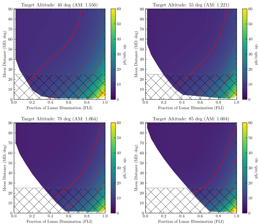
Figure 19: Estimated sky background in photons per sub-aperture in the LGS low-order wavefront sensor at 250Hz as a function of fraction of lunar illumination (FLI) and Moon distance (MD) for four different target elevations. Red contours denote recommended maximum Moon background levels for guide stars between 17th and 15th magnitude. The hatched region denotes Moon distances that are not permitted due to issues with telescope guiding. Due to geometry it is not possible for a Moon with FLI \sim 0 to be close to the zenith at night.
