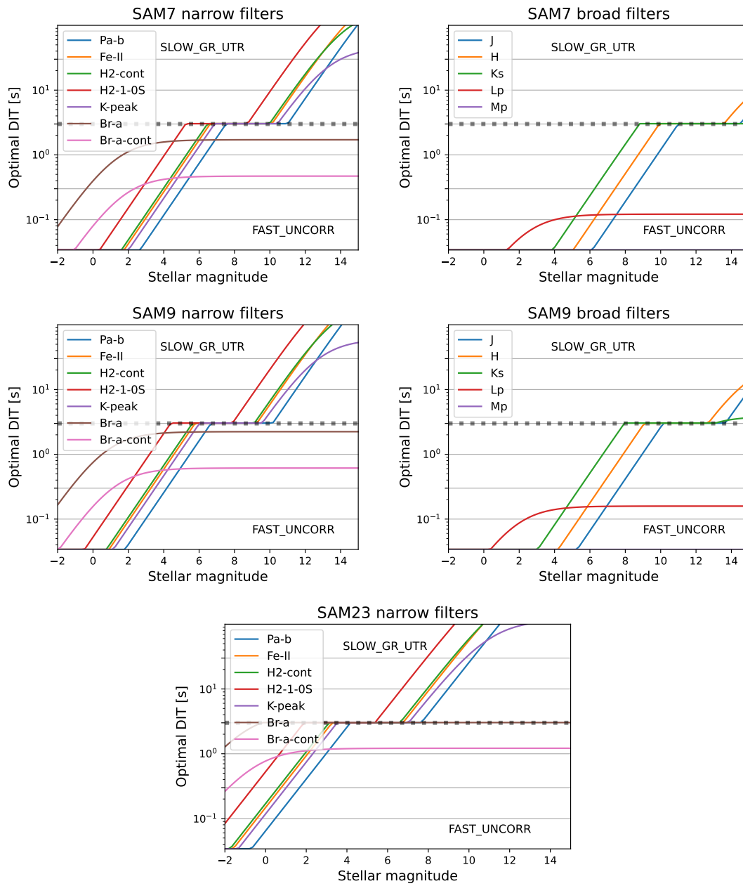
Figure 29: Optimal DIT used in combination with each SAM mask and each filter as a function of stellar magnitude of the target. These values were derived from the ERIS ETC.
