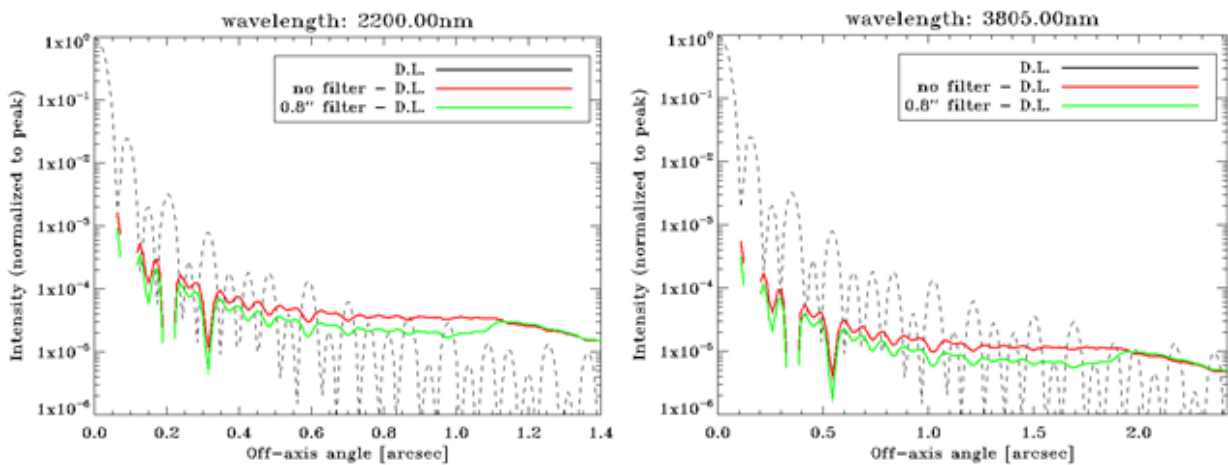
Figure 24: The corrected PSFs profiles at K and L' band for the two options baseline and filtered SH for the NGS WFS. Different behavior is given by red and green line respectively. DL in the figure labels means Diffraction Limit.
