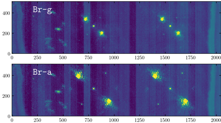
Figure 31: A composite image of the acquisition position for APP observations (800, 1536), and the recommended offset position at (1550, 1536) within the recommended window4 sub-array for K -band (top) and L -band (bottom).
