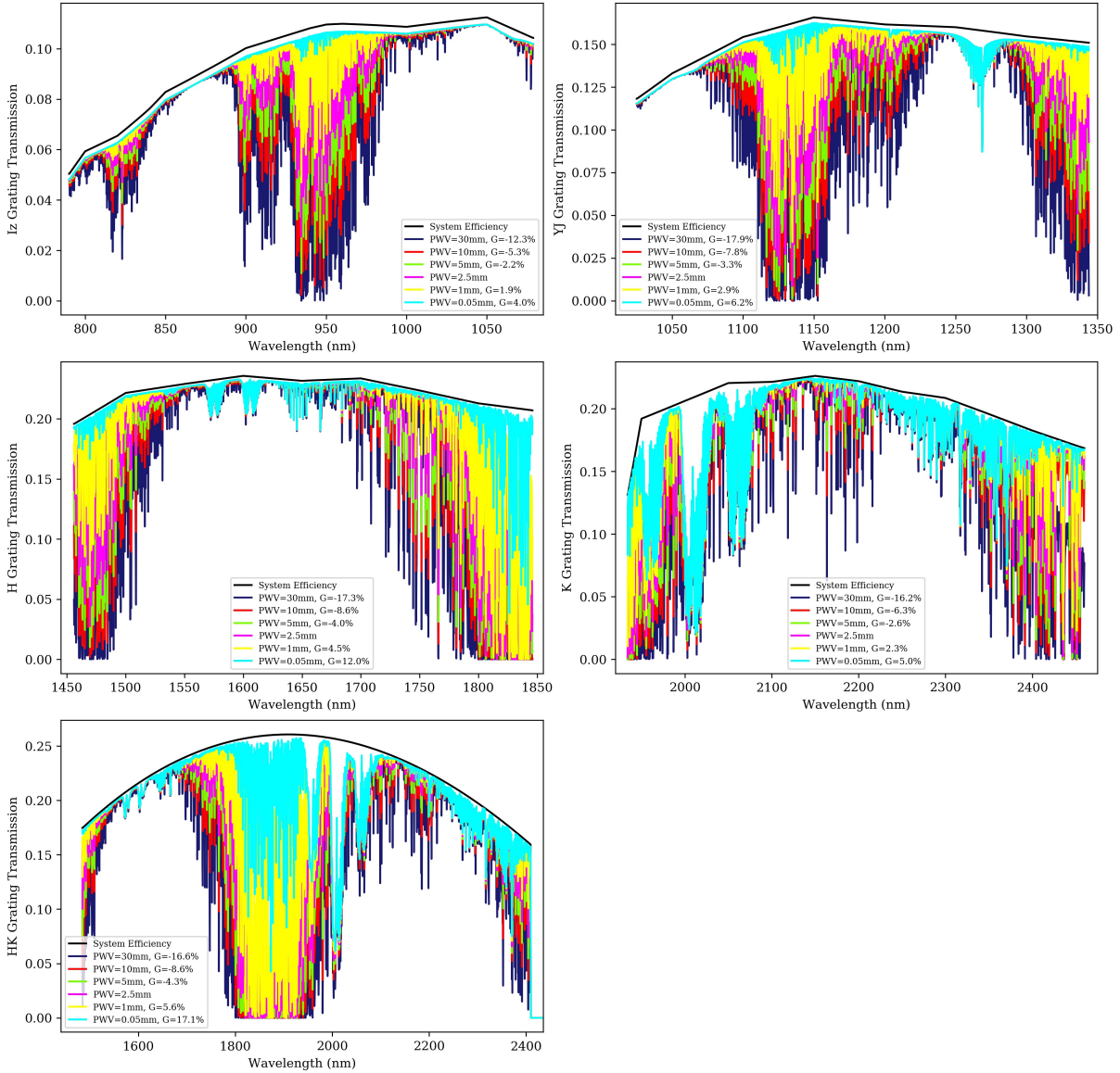
Figure 16: Effect of PWV on the transmission curves of the IZ-, YJ, H-, K- and HK-gratings. The black curves denote the transmission curves without atmosphere effects, and the coloured curves represent the transmission curves convolved with the sky transmission at different PWV values, as indicated. PWV=2.5mm (pink curve) is used as a reference value to compute the gain (G) in total transmission for different PWV conditions.
