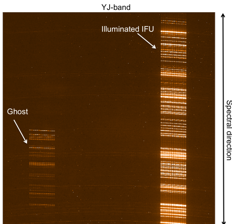
Figure 18: Image in the YJ-band, with one single IFU illuminated with a Argon+Neon calibration lamp (on the right). The ghost is visible on the left side of the array. The colour scale has been enhanced to show the ghost, since the level of the ghost is less than 1% for all bands.
