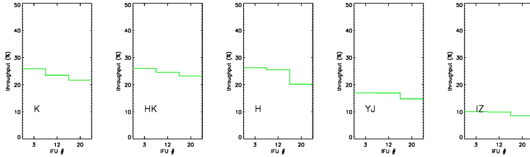
Figure 24: Total instrument transmission for the three detectors and all five bands.
