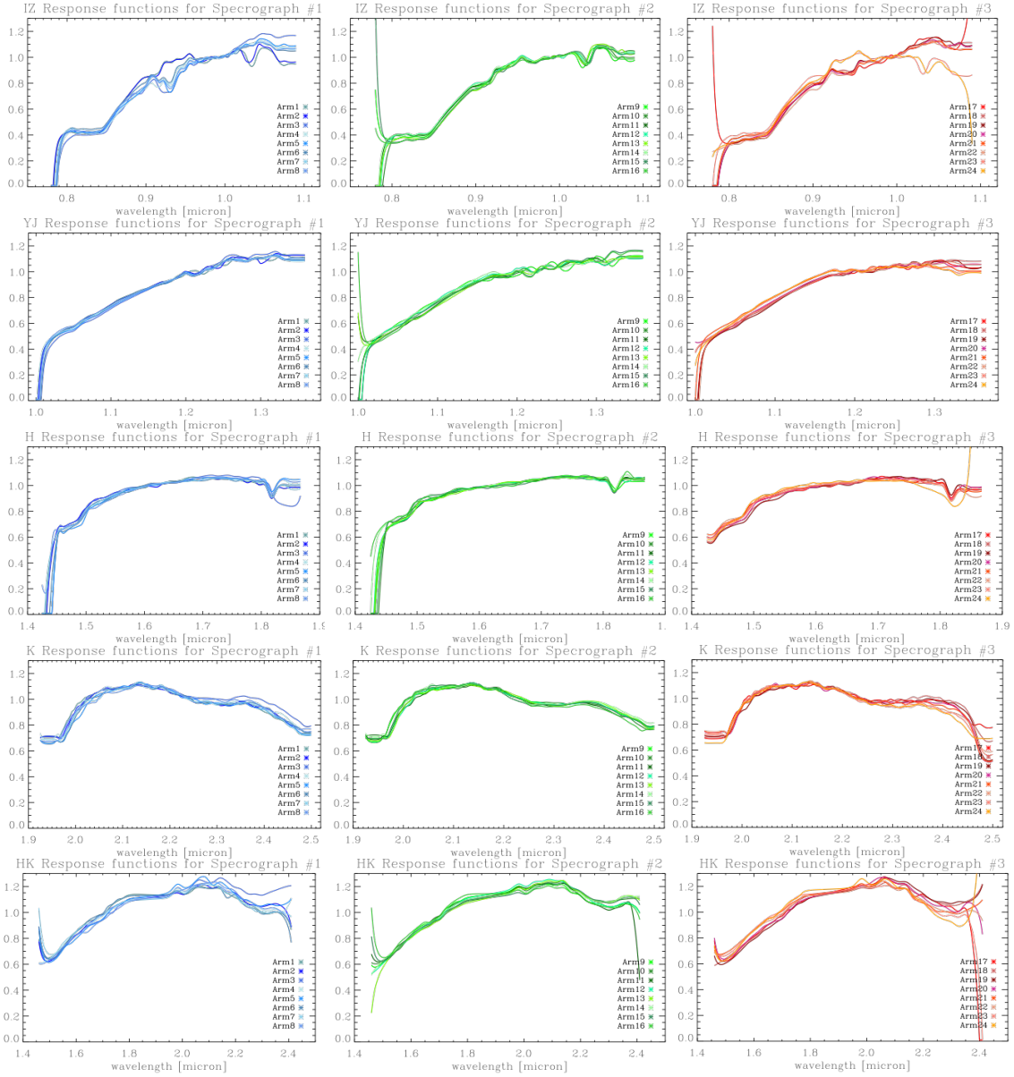
Figure 25: Response function as a function of wavelength obtained per arm and per grating. Ordinates are in arbitrary units.
