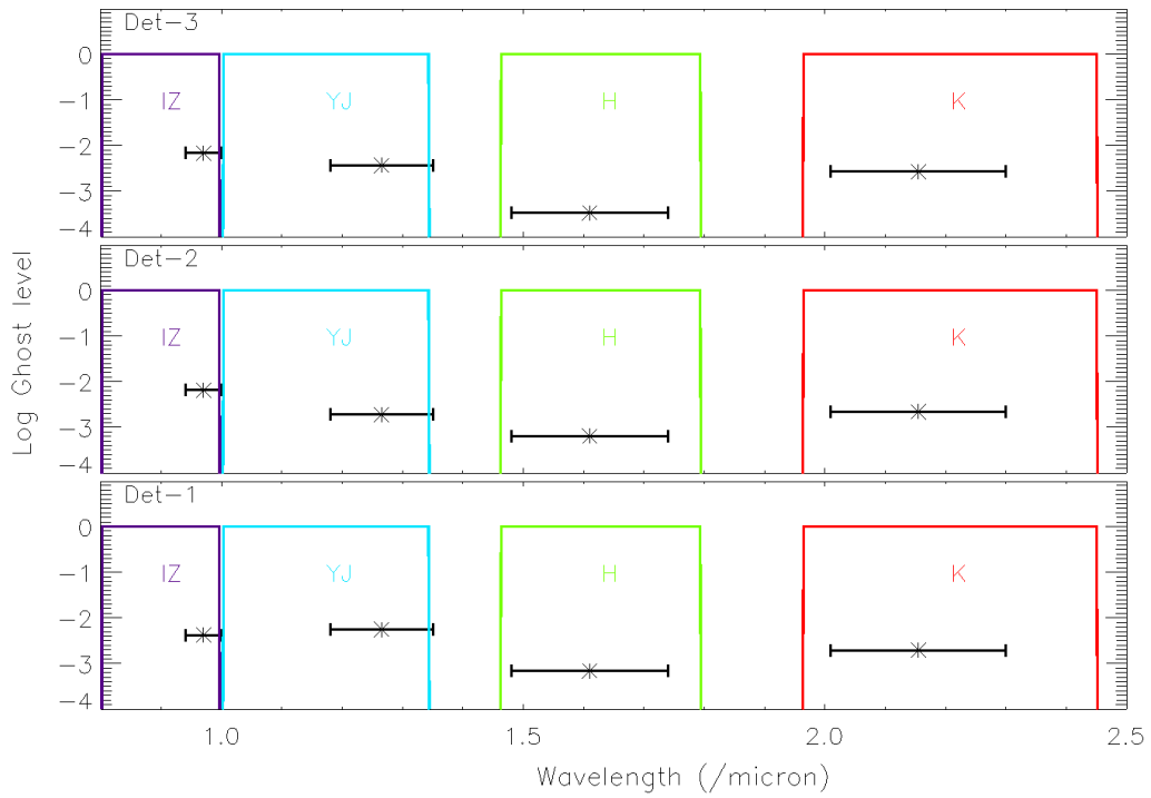
Figure 19: Ghost level as a function of wavelength, for all three detectors. The ghost level is defined as the intensity of the ghost image divided by the intensity of the source that has generated it. The coloured boxes identify the full wavelength coverage in each band (IZ, YJ, H, K). The horizontal error bars denote the fraction of the band affected by the ghost. It can be noted that the level is less than 1 part in 100 and only affects a fraction of the wavelengths, especially in the IZ and YJ bands. The ghost is not present in the HK band.
