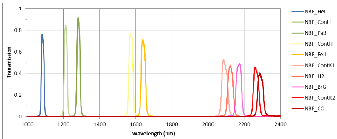
Figure 46: IRDIS NB filters.
