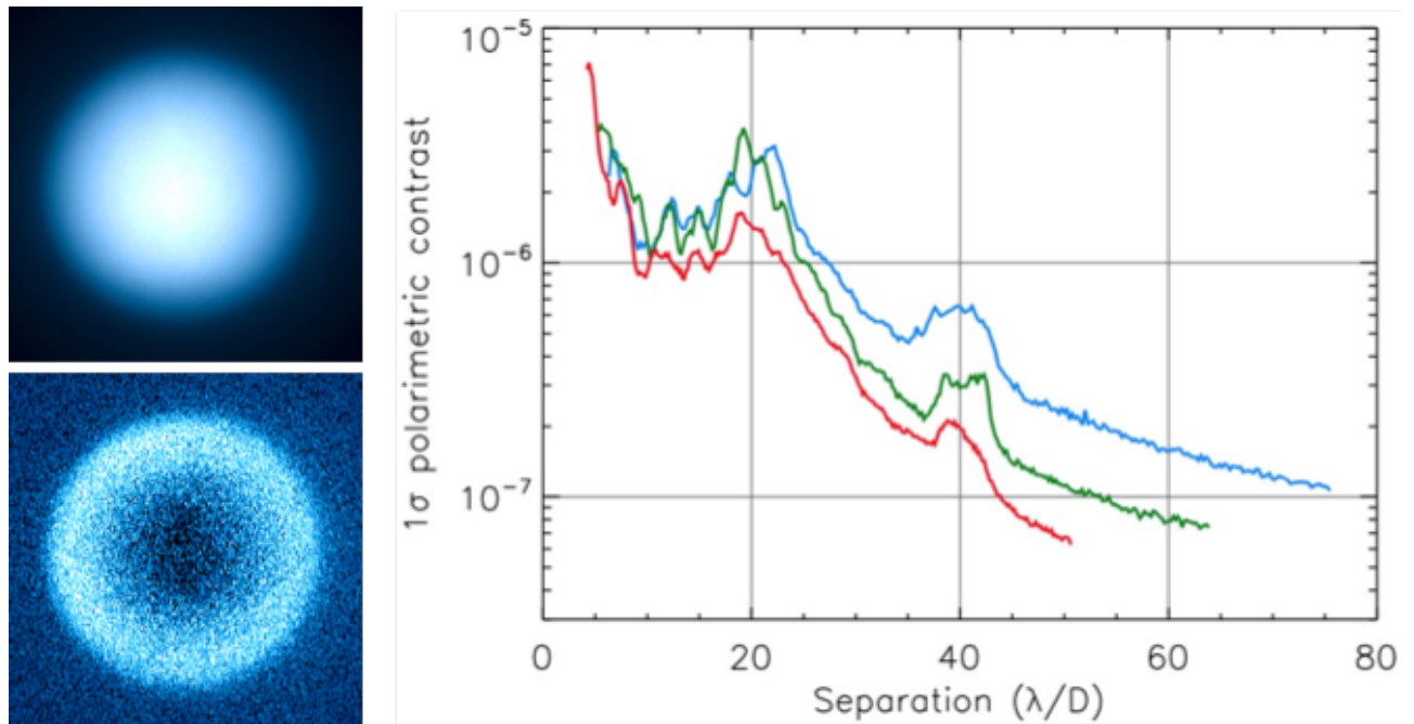
Figure 23: Top left: intensity image of Titan. Bottom Left: polarized intensity. Right: polarimetric contrast (right) on a bright target for the V (blue), N_R (green), N_I (red) filters.
