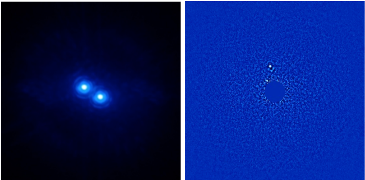
Figure 22: Left: High angular resolution imaging of a binary (150 mas separation) as seen by ZIMPOL in I band. Right: Pupil-stabilized ZIMPOL imaging providing ADI contrast close to 12 mag at 0.2'' (previously unknown companion).
