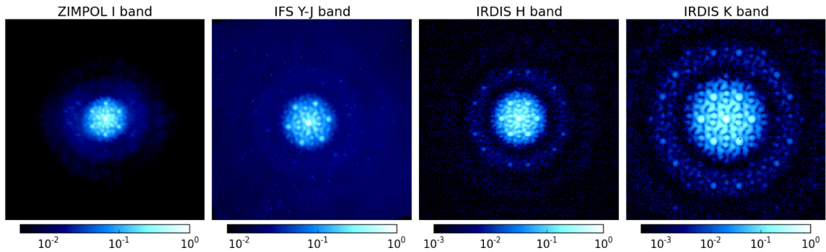
Figure 24: SAM_7H on-sky point spread functions for 4 observing wavelengths with 3 cameras: a ZIMPOL I band exposure, a IFS wavelength slice between Y and J bands, an IRDIS H band image and an IRDIS Ks band image.
