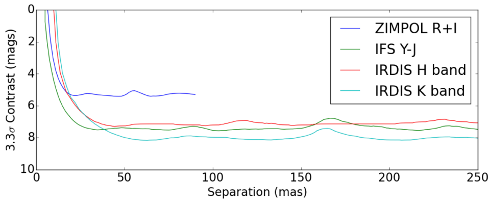
Figure 26: SAM_7H contrast limits for the detection of companions in various bands from the test data (July 2015). Each dataset consisted of approximately 1hr in execution time, including time for observations of calibrator stars. This was obtained on the F6 star HD142527 with R=8.3, J=6.5, H=5.7, K=4.98 with a seeing \sim 0.6-0.8'' . HIP113246 and HD169319 were used as calibrator stars (Cheetham et al., in prep.).
