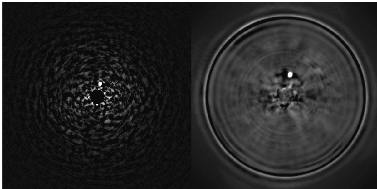
Figure 20: Detection in parallel by IRDIS (left) and IFS (right) of a faint companion at 0.24'' around the bright star HR7581 (see ESO Press Release 1417, http://www.eso.org/public/news/eso1417/ ).
