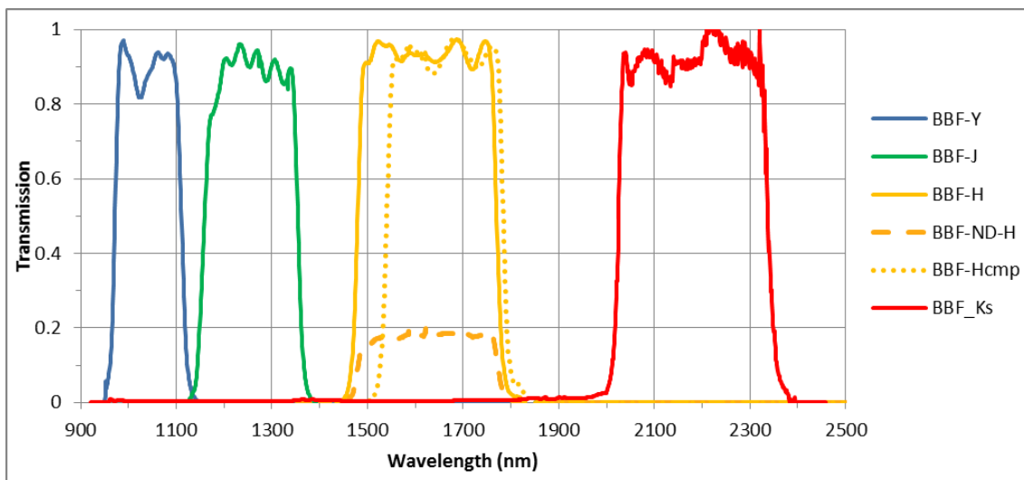
Figure 44: IRDIS BB filters.
