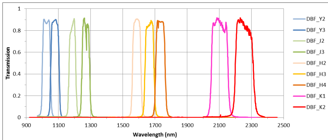
Figure 45: IRDIS DB filters.
