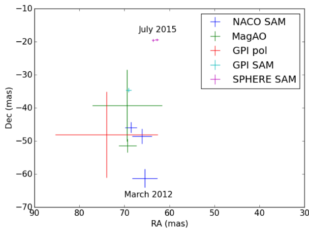
Figure 27: SAM_7H astrometry of the low-mass star companion HD142527B with respect to its host: the position uncertainty ( \sim 0.6 mas at 70 mas separation) is superior to the one obtained by other instruments and at different epochs (Cheetham et al., in prep.).
