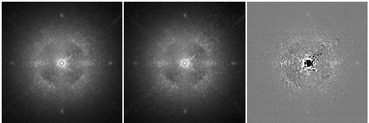
Figure 15: Coronagraphic images obtained in IRDIS H2 (left) and H3 (center) DBI filters, and the result of spectral differential imaging H2-H3 (right).
