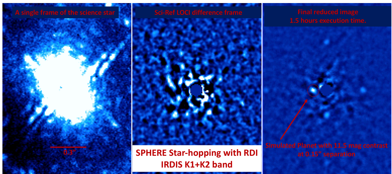
Figure 34: Reduced images from a star-hopping RDI data set. Left: a single DIT=16s image of the target star. Middle: The corresponding difference image after RDI. Right: The final RDI reduced image after derotation and coadding. A simulated planet, implanted with contrast 11.5 mags at 0.15'' separation is recovered after reduction. No spectral differencing was done. The K1 and K2 channels were added together, and the simulated planet was given the same contrast in the two channels. All images show the same intensity range in square-root stretch. The images are 0.8'' \times 0.8'' . See Wahhaj et al. 2021 for more details.
