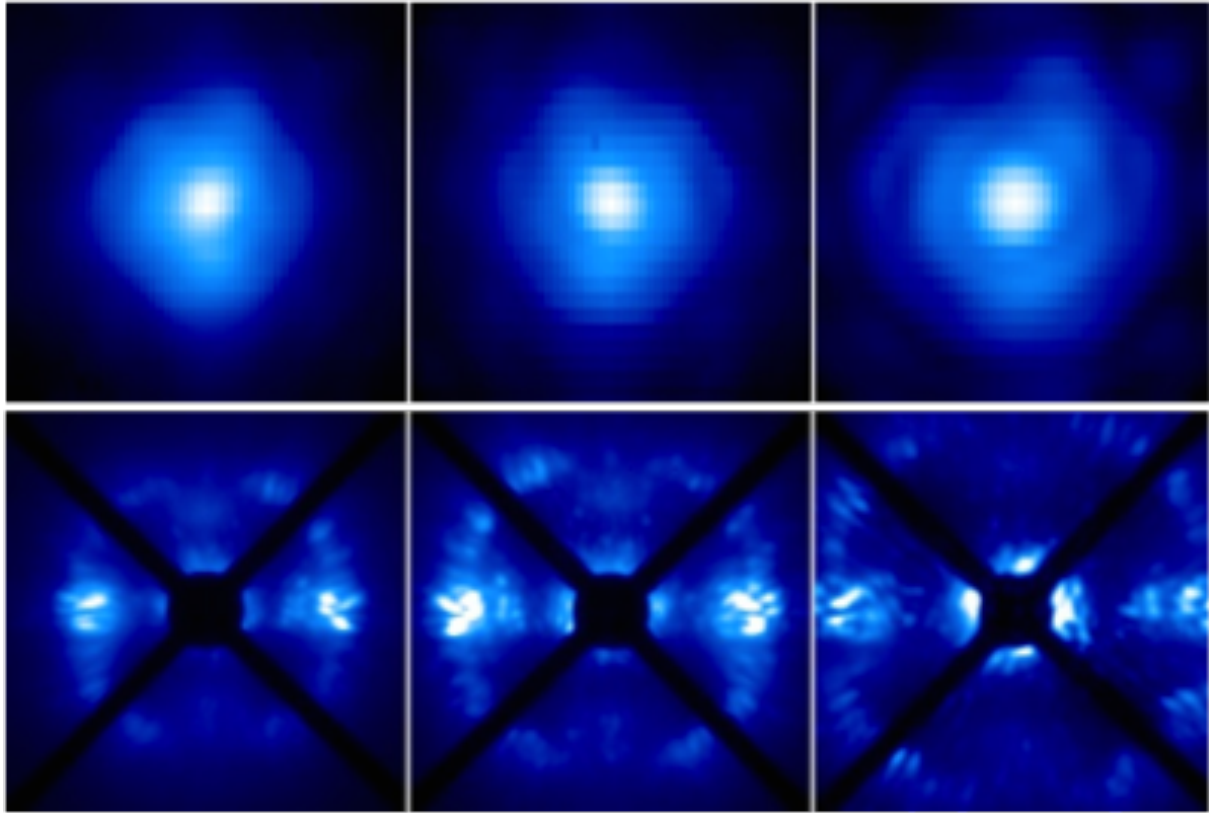
Figure 21: PSF (top) and coronagraphic (bottom) images of ZIMPOL in V, N_R, N_I filters.
