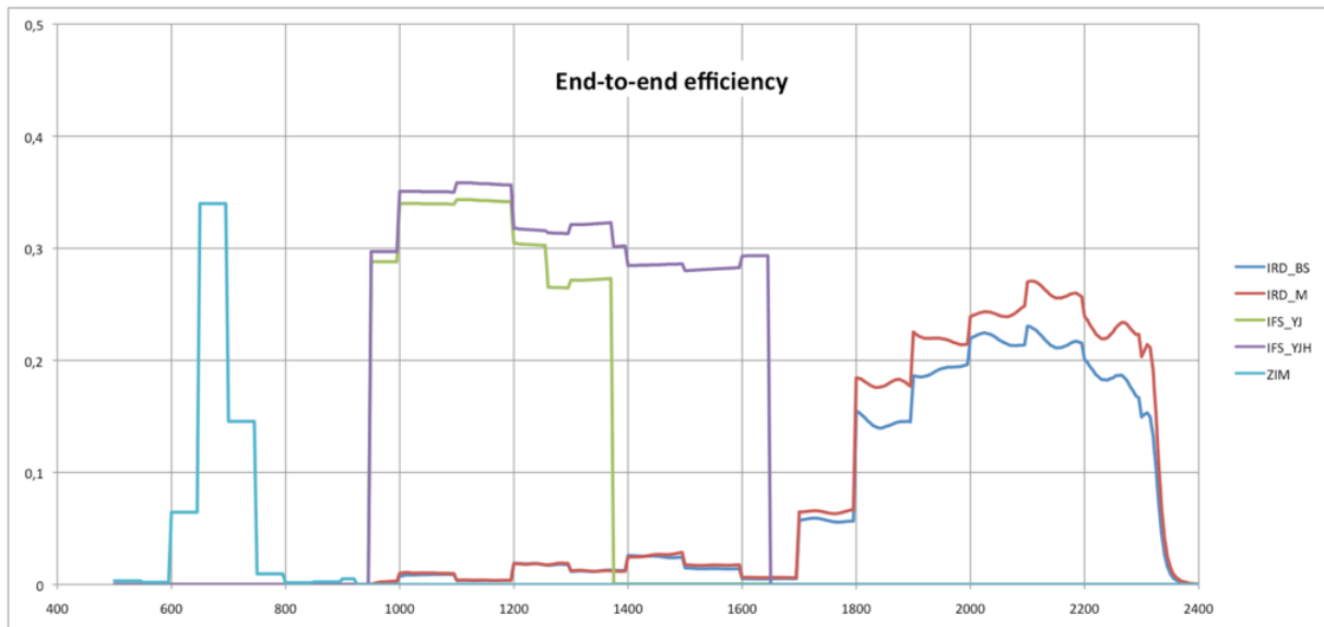
Figure 39: Transmission (as above) with different beamsplitters. In visible: separation between WFS and ZIMPOL uses a dichroic sending more light to ZIMPOL but in R band only; in NIR: the IFS/IRDIS dichroic ‘K’ feeds IFS with the its full Y-H range, with lower efficiency for IRDIS in K band only.
