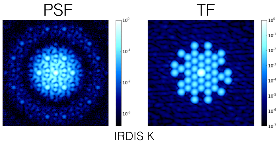
Figure 25: An image (left) produced by the aperture mask. For the 7 hole mask, the PSF is a combination of 21 sets of interference fringes. The phase and amplitude of each baseline contains information about the structure of the object being observed. The Fourier Transform of the previous image (right) allows to work in the Fourier space. Each set of interference fringes has a different frequency and direction, and so they are well separated in Fourier space and the phase and amplitude of each can be measured directly.
