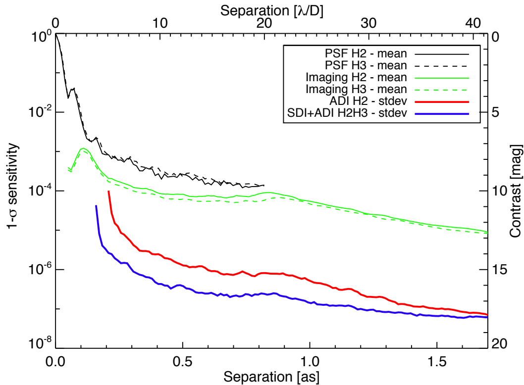
Figure 16: IRDIS DBI H2H3 contrast curves obtained on-sky for a bright target ( H=0.2 ), in average conditions (seeing \sim 1.0'' ), with an ADI field rotation of 30 degrees. The plot shows the PSF profiles (black) and coronagraphic profiles (green) in the H2 and H3 filters, the 1\sigma contrast curve for ADI on the H2 data (red), and the 1\sigma contrast curve for SDI+ADI on the H2 and H3 data. For the ADI and SDI+ADI analysis, the algorithm throughput is taken into account and compensated, assuming a T8 spectral-type for the planet in SDI.
