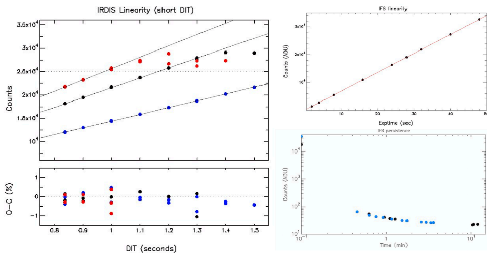
Figure 37: IRDIFS linearity and persistence
