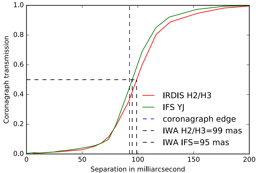
Figure 48 Transmission profile for the N_ALC_JYH_S coronagraph
