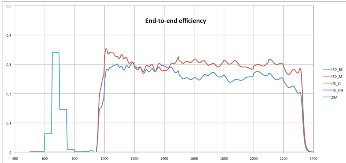
Figure 40: Transmission (as above) in IRDIS alone configuration where all the NIR light is sent to IRDIS.
