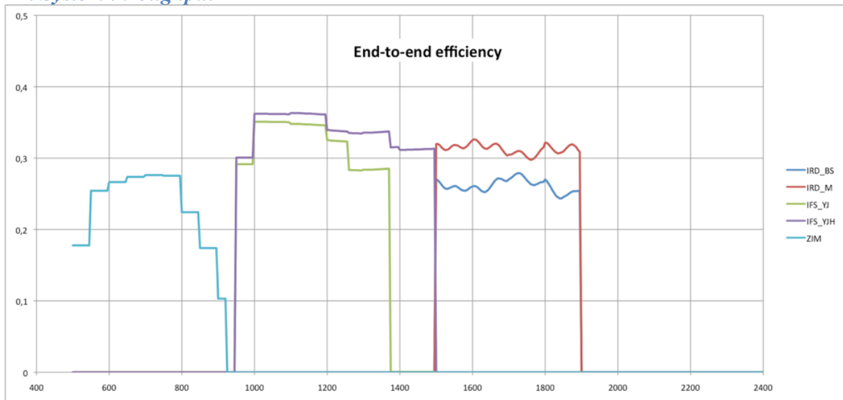
Figure 38: Transmission from SPHERE entrance to the science detectors, including the detector efficiency, assuming i) no coronagraph, ii) ZIMPOL path goes through the GREY beamsplitter (80% to ZIMPOL), and iii) the H dichroic separating the flux between IFS (up to 1450 nm) and IRDIS. Note that IRDIS cannot observe in K band in this setup.
