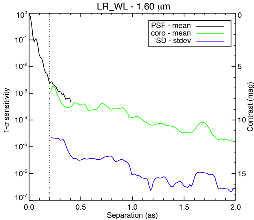
Figure 18: IRDIS LRS 1\sigma sensitivity curve at 1.6\ \mu\text{m} obtained on PZ Tel ( H=6.5 ). The plot shows the PSF profile (black), the coronagraphic profile (green) and the noise level after subtraction of the stellar halo and speckles using spectral difference (SD). The dotted vertical line represents the edge of the coronagraphic mask. At a separation of 0.5'' , the raw contrast in LRS data is 2\text{-}5 \times 10^{-4} , and the speckles can be estimated and subtracted down to a level of a few 10^{-6} . However, this noise level curve does not completely represent the capabilities of IRDIS LRS mode, because one has to consider that the final characterization performance is defined by the overall quality of the spectral subtraction, and not only by the noise level in a single spectral channel, which is always optimistic. A safety margin of a factor 3 to 5 with respect to these limits has to be taken into account when foreseeing LRS observations.
