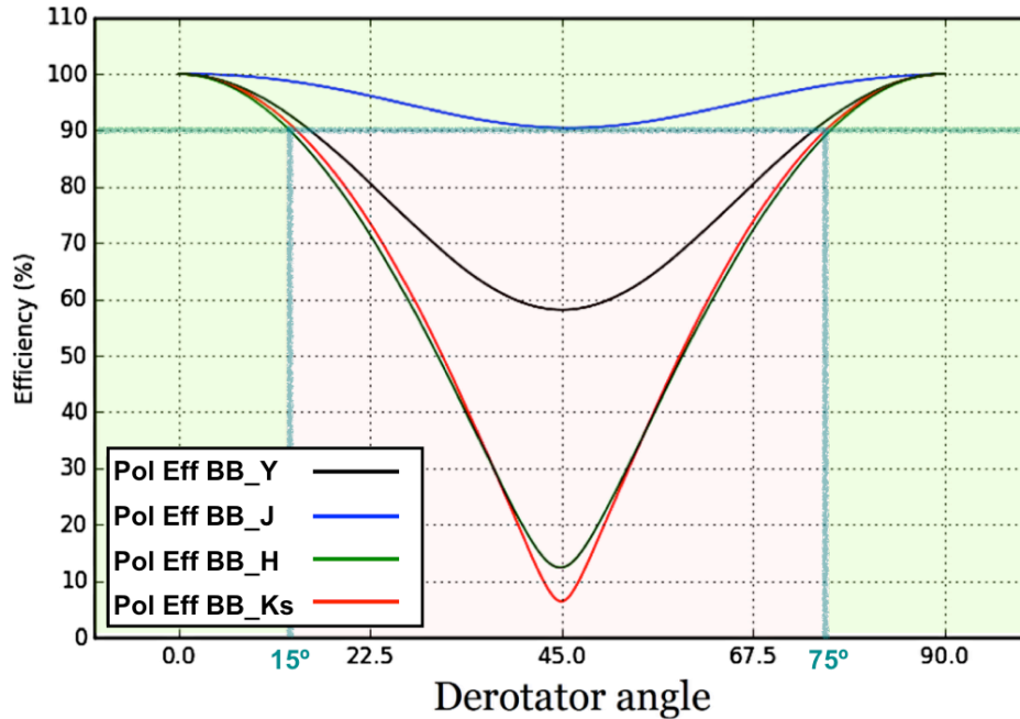
Figure 35: Measurements of the instrumental polarization efficiency (not accounting for the telescope) for four broad band filters. For best use of the DPI mode (relevant for field tracking while irrelevant for pupil tracking), one should avoid the pink zone where the efficiency drops below 90% (> 10% loss due to cross-talks). For that, one should make sure the derotator angle stays < 15° or > 75°. J-band is the least affected and therefore the most recommended filter, especially for long observations featuring a large parallactic angle variation. At J-band the efficiency is always > 90%.
