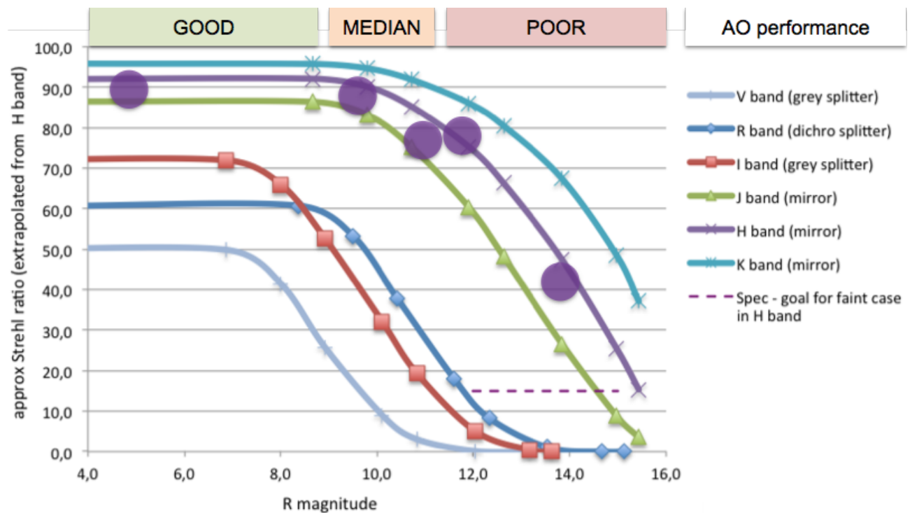
Figure 11: Theoretical and measured (purple circles) SPHERE-SAXO Strehl ratio as a function of R magnitude for good seeing conditions and different wavelength ranges from V to K (see Figure 31 and Figure 32 for more details).
