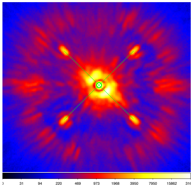
Figure 49. Irdis image in broad-band H, with the N_ALC_YJH coronagraph, with the waffle pattern applied to the DM, creating four satellite spots. These spots are elongated with broad-band filters and point source with narrow-band filters. The green lines start and end points were computed by fitting a 2D Gaussian on each spot, they intersect on the star center, indicated by a green thick circle.
