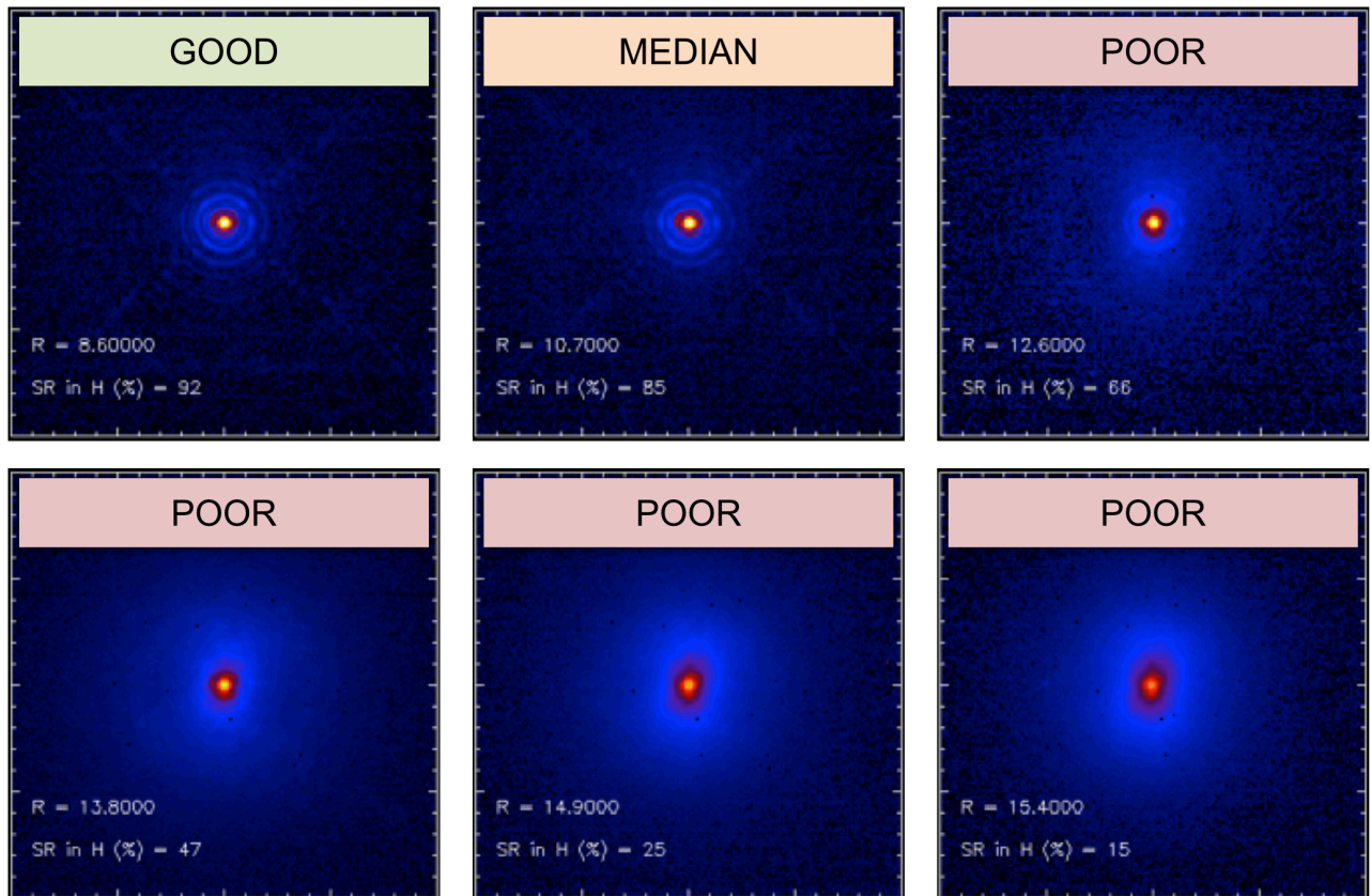
Figure 12: SPHERE PSF morphology and Strehl ratio as a function of R magnitude (see Figure 31 and Figure 32 for more details).
