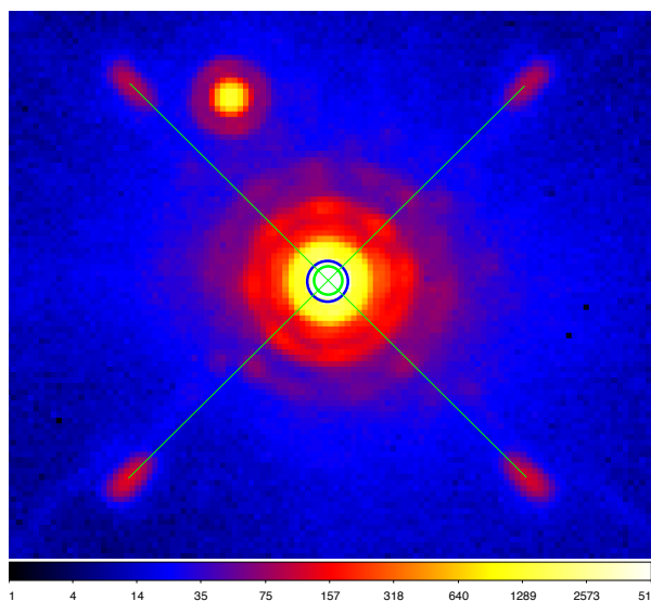
Figure 50 Non coronagraphic image of a star (happening to have a binary companion) in broad-band H with Irdis, after applying a waffle pattern to the DM for calibration purposes. The green thick circle indicates the intersection of the green lines, while the blue thick circle indicates the star position (Gaussian fit). Both agree within 2.5mas.
