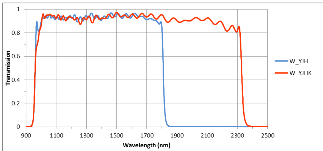
Figure 47: IRDIS wideband filter.
