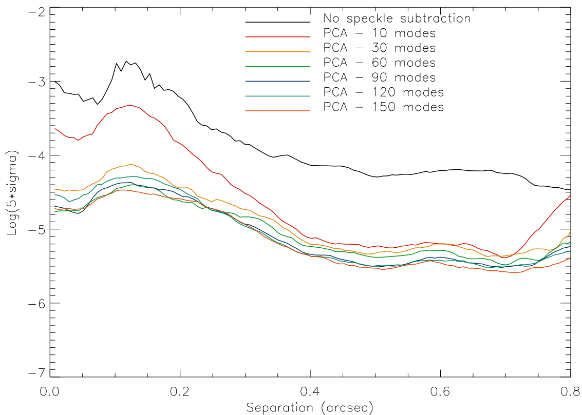
Figure 19: IFS 5\sigma sensitivity on Iota Sgr as function of angular separation, for different principal components retained in the speckle subtraction using both spectral and temporal diversity (ADI).
