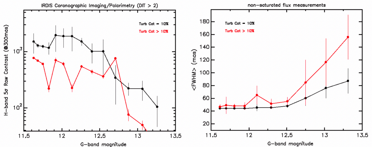
Figure 13: (Left) Single image IRDIS contrast versus Gmag. (Right) PSF core FWHM versus Gmag. Both H-band contrast and image resolution degrade quickly for targets fainter than G=12.5.
