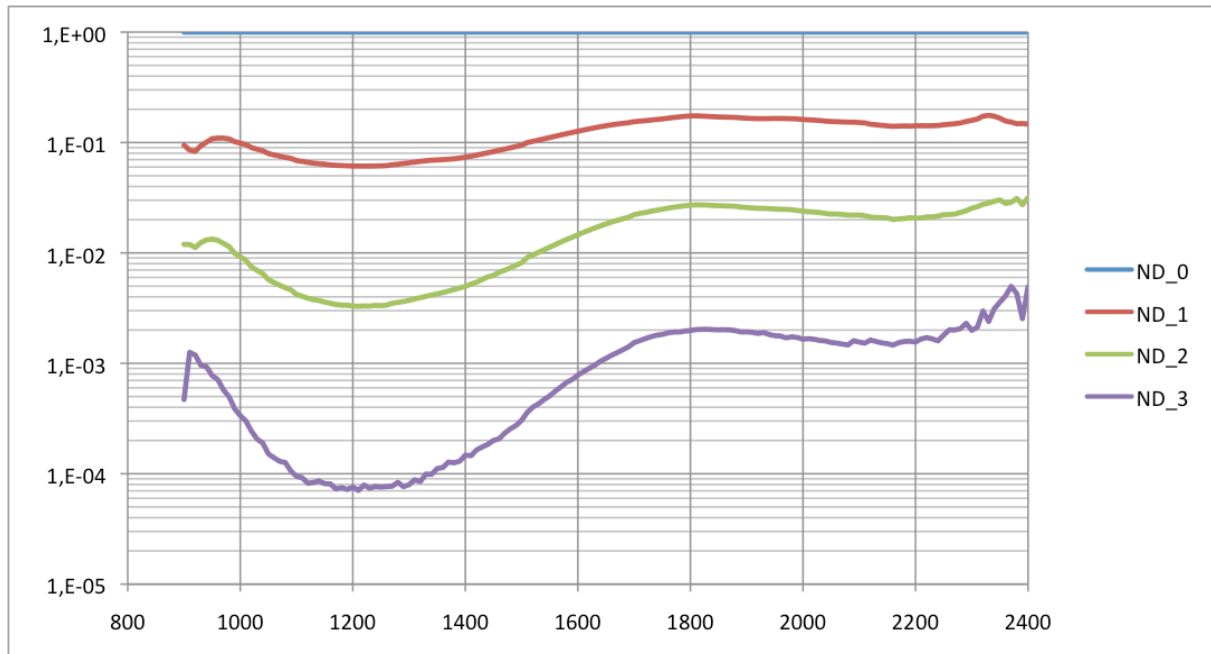
Figure 41: Transmission CPI NIR densities as a function of wavelength (nm).
