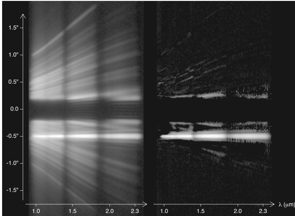
Figure 17: IRDIS LRS data obtained on PZ Tel (H=6.5). The left image is the spectrum after preprocessing and cleaning using the data reduction and handling pipeline (DRH). It corresponds to a 20 minutes exposure (DITxNDITxNEXP=20x10x6) in good conditions (seeing of 0.5'' - 0.6'' ). The spectrum of the companion PZ Tel B is visible as a straight line amidst the speckles at an angular separation of \sim 0.5'' . The obscured part between \pm 0.2'' corresponds to the position of the opaque coronagraphic mask. The contrast of the companion is \sim 5.4 mag in H-band (Biller et al. 2010, ApJ, 720, 82). The right image is the data after stellar halo and speckles subtraction using the spectral difference approach described in Vigan et al. 2008 (A&A, 489, 1345). The spectra are displayed with the same logarithmic color scale.
