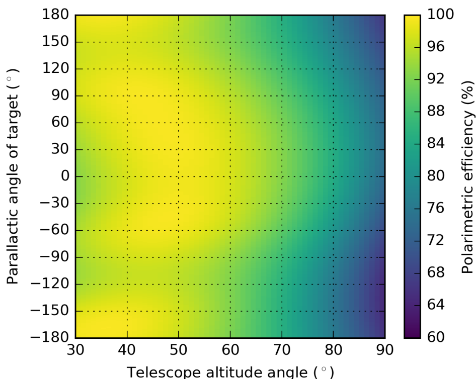
Figure 32b: Polarimetric efficiency for pupil-tracking in H-band as a function of parallax and altitude angle (van Holstein et al. 2017, SPIE)
