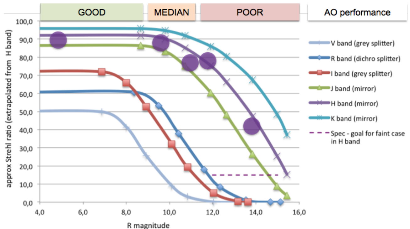
Figure 11: Theoretical and measured (purple circles) SPHERE-SAXO Strehl ratio as a function of R magnitude for good seeing conditions and different wavelength ranges from V to K (see Figure 31 and Figure 32 for more details).
