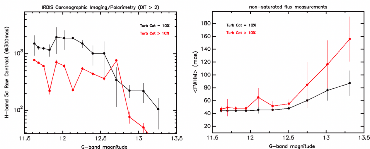
Figure 13: (Left) Single image IRDIS contrast versus Gmag. (Right) PSF core FWHM versus Gmag. Both H-band contrast and image resolution degrade quickly for targets fainter than G=12.5 (Jones et al. 2022).
