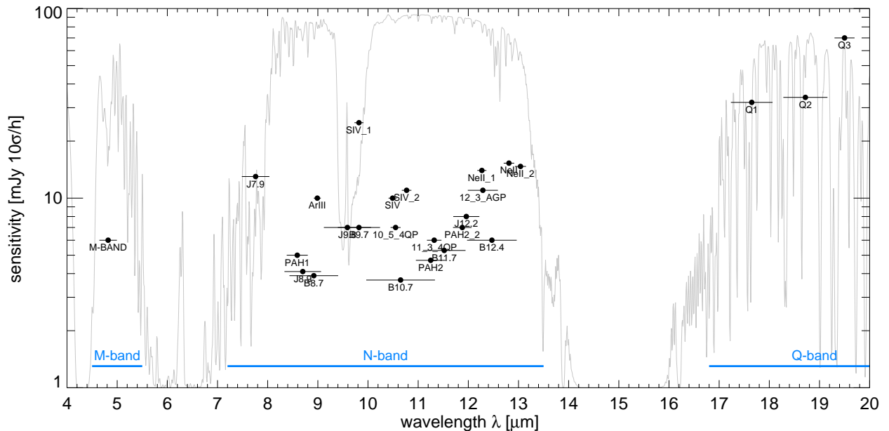
Figure 6: Sensitivities for the VISIR imager in various filters in the M-, N- and Q-bands determined with the new AQUARIUS detector. The atmospheric transparency spectrum for PWV = 1 mm at an airmass of 1 is plotted in the background.
