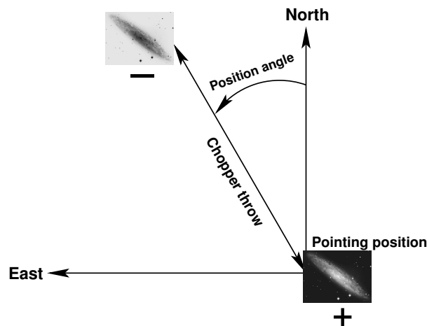
Figure 17: Definition of chopping parameters from the telescope point-of-view. The (chopping) position angle ( TEL.CHOP.POSANG ) is measured counter-clockwise from North to East, between 0^\circ and 360^\circ . The positive beam (+) is obtained when the M2 is at Chopping Position A and corresponds to the pointing position of the telescope as given in the FITS header (idle position). The negative beam (-) is obtained by moving the M2 so that it points to a position angle on the sky given by TEL.CHOP.POSANG and a throw of TEL.CHOP.THROW from the telescope pointing position (Chopping Position B). If TEL.CHOP.POSANG = TEL.ROT.OFFANGLE , the resulting image on the detector will appear as in one of the nodding position images illustrated in Fig. 19.
