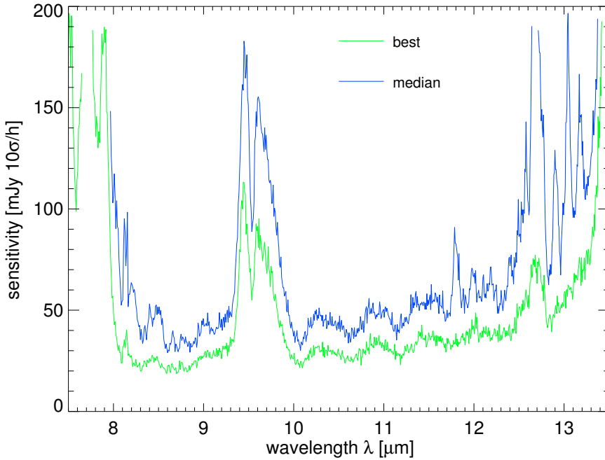
Figure 10: Median and best low resolution sensitivities [mJy/10 \sigma /h] observed during commissioning 2 under mediocre atmospheric conditions.
