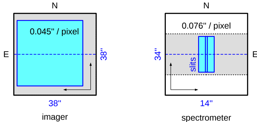
Figure 16: Field orientation and pixel scale for the imaging (SF) and the spectroscopic modes of VISIR for TEL.ROT.OFFANGLE = 0° . While the imaging detector follows the normal astronomical convention, the spectroscopic detector is reversed in x -direction so that East is to the right. The gray area marks the region of the detector which is typically read-out, the spectroscopy detector being windowed in y -direction. The magenta areas mark the areas illuminated by the sky – in case of the spectrometer for the very wide slit (“OPEN”). The sizes of these usable areas on sky are given in blue (see also § 3.4).
