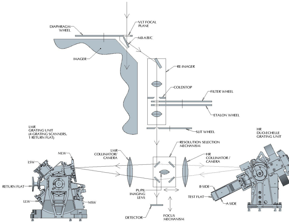
Figure 9: Schematic layout of the design of the VISIR spectrometer.
