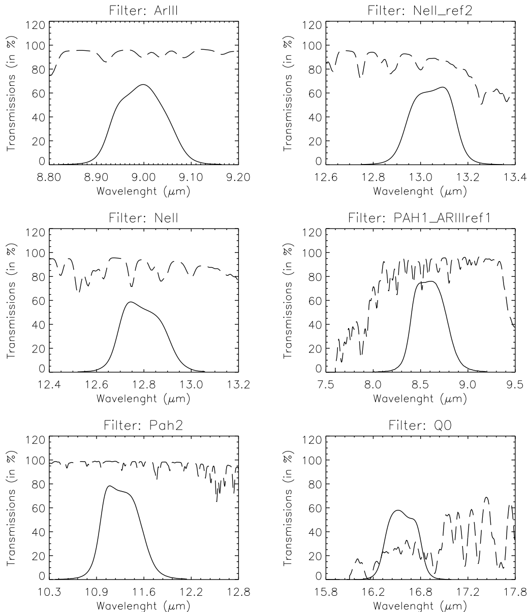
Figure 23: Transmission curves of VISIR imager filters, manufactured by READING. Overplotted (dashed) is the atmospheric transmission at low resolution. The absolute transmission values are given, expressed in percent.
