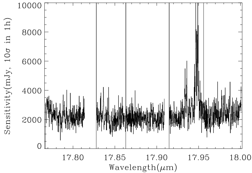
Figure 33: Measured on the old DRS detector. Observed sensitivity as a function of wavelength for high resolution mode. Offered sensitivity is typically a factor of 2 larger.
