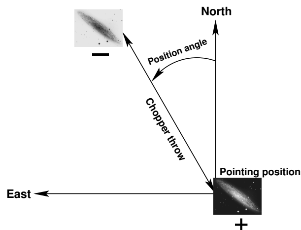
Figure 12: Definition of chopping parameters from the telescope point-of-view. If the position angle ( PA ) is measured counter-clockwise from North to East with PA between 0 and 360^\circ , then TEL.CHOP.POSANG is 360^\circ - PA . The positive beam (+) is obtained when the M2 is at Chopping Position A and corresponds to the pointing position of the telescope as given in the FITS header (idle position). The negative beam (-) is obtained by moving the M2 so that it points to a position angle on the sky given by PA and a throw of TEL.CHOP.THROW from the telescope pointing position (Chopping Position B). If TEL.CHOP.POSANG = TEL.ROT.OFFANGLE = 360^\circ - PA , the resulting image on the detector will appear as in one of the nodding position images illustrated in Fig. 14.
