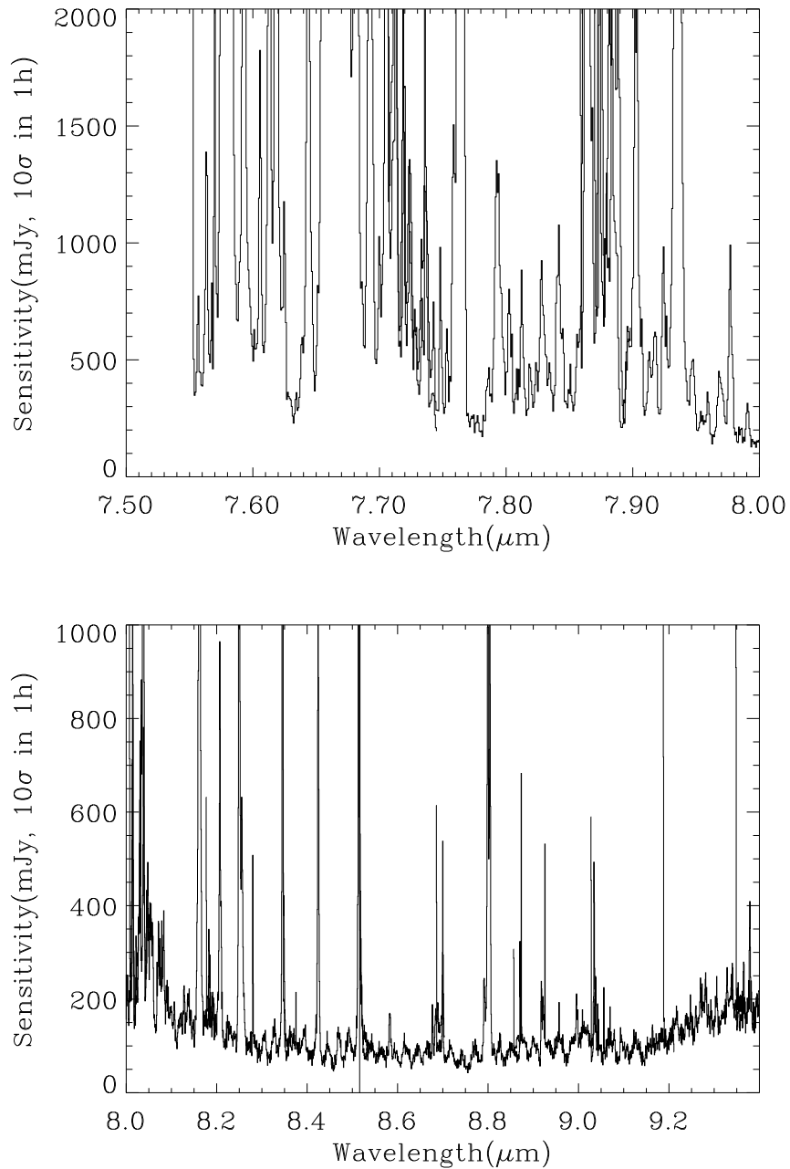
Figure 21: Measured on the old DRS detector. Observed sensitivity as a function of wavelength for different settings in the medium resolution mode obtained in very good weather conditions: (I) for 7.5\mu\text{m} < \lambda < 9.4\mu\text{m} . Offered sensitivity is typically a factor of 2 larger.
