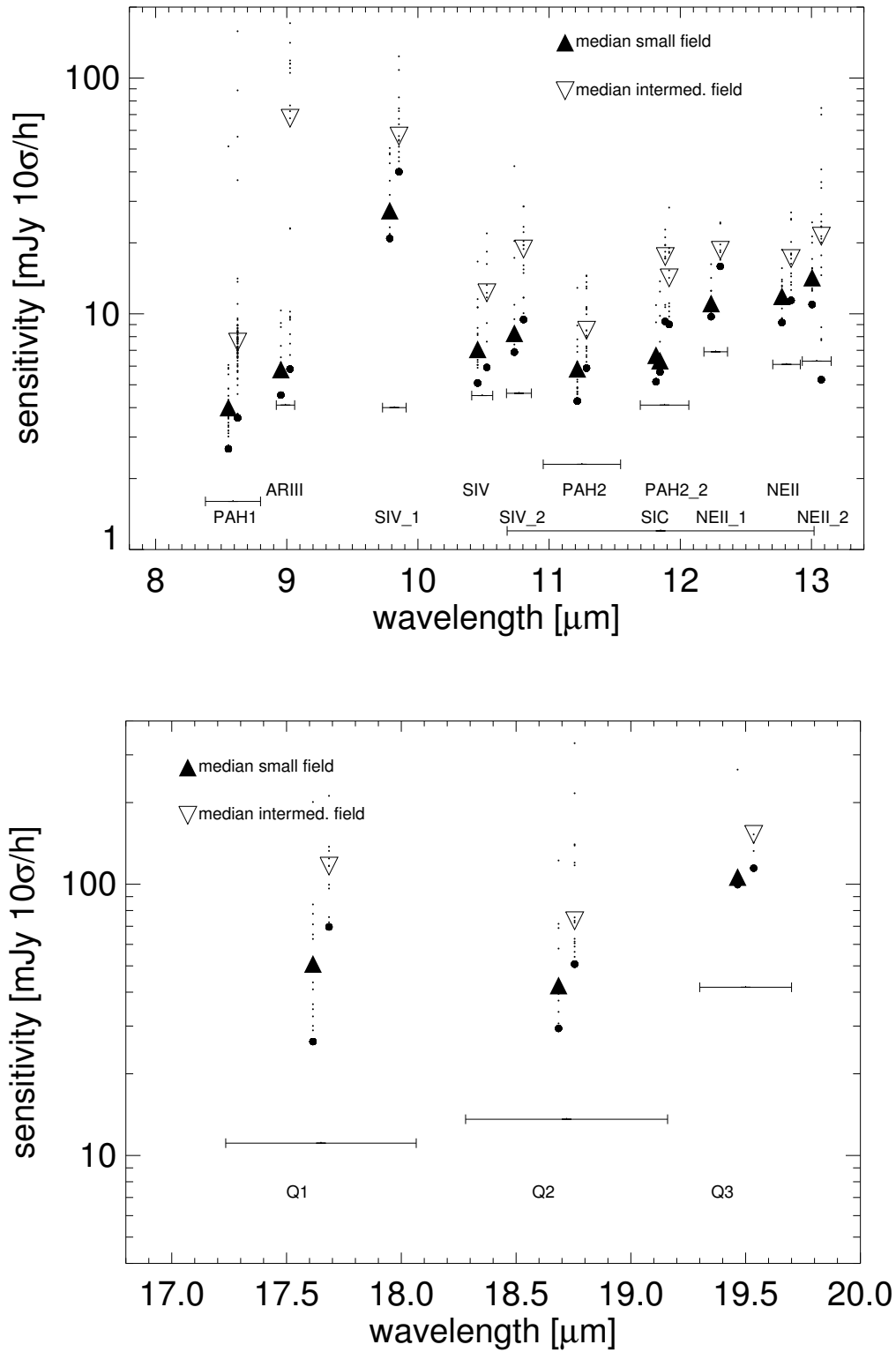
Figure 5: Measured on the old DRS detector but also valid for Period 89. Sensitivities for the VISIR imager for the N (top) and Q-band (bottom). Small and intermediate field observations are displaced for clarity. Background noise limits are indicated for the individual filter bandpasses.
