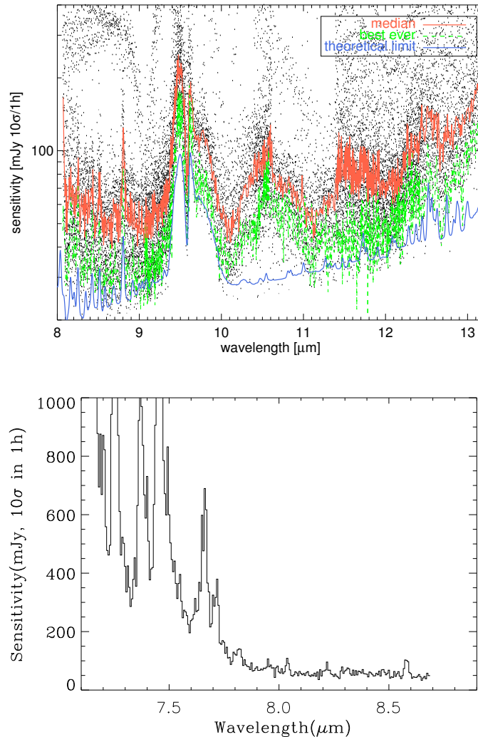
Figure 20: Measured on the old DRS detector. Sensitivity as a function of wavelength for low resolution mode. Top: Four offered settings of the N-band low-resolution are stitched together. Atmospheric molecular absorption, e.g. at 9.55, 11.8 and 12.5 \mu\text{m} , is evident. Note the detector feature at 8.8 \mu\text{m} . Dots indicate individual observations, full lines represent median and the dashed line the best sensitivities. Theoretical model curves correspond to BLIP. Bottom: Sensitivity measured in the bluer setting, centered at 8.1 \mu\text{m} .
