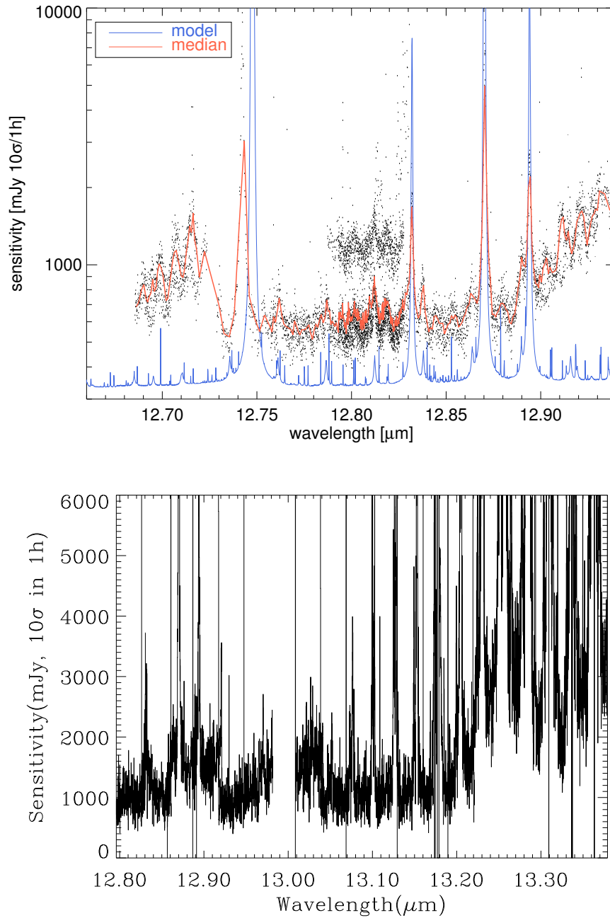
Figure 30: Measured on the old DRS detector. Observed sensitivity as a function of wavelength for high resolution mode. Top: Observed sensitivities obtained on various nights, compared with the theoretical model curves, corresponding to BLIP. Bottom: Sensitivities over an extended region encompassing the observed wavelength of [NeII] up to z \approx 0.038 .
