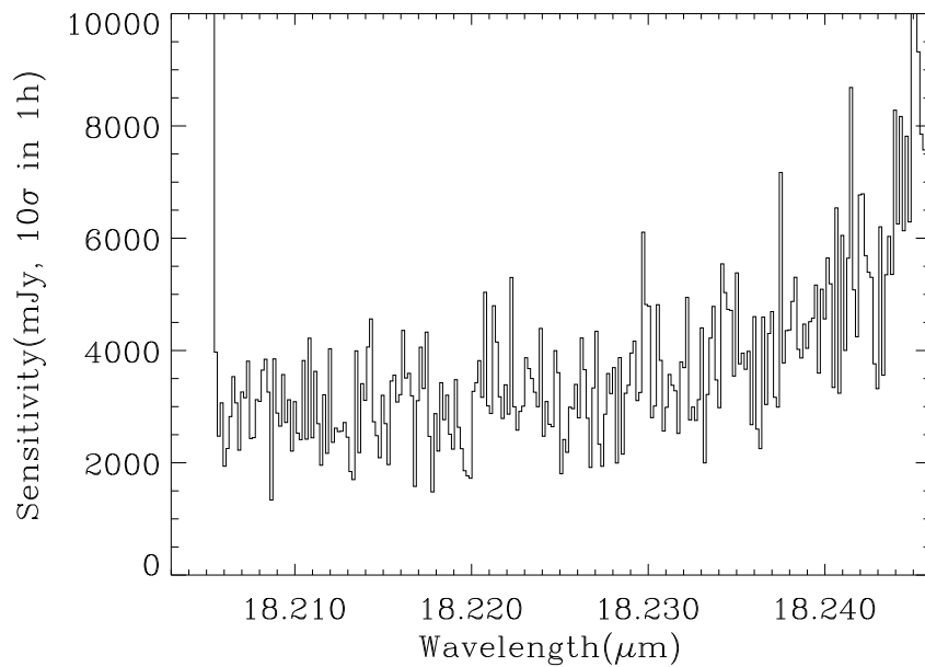
Figure 34: Measured on the old DRS detector. Observed sensitivity as a function of wavelength for high resolution mode. Offered sensitivity is typically a factor of 2 larger.
