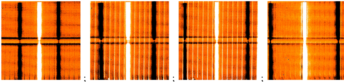
Figure 9: An example of the bad cosmetics on the old DRS detector. Sequence of chop/nod, reduced spectra obtained in the Medium Resolution mode with a central wavelength = 8.8\mu\text{m} . The TEL.CHOP.THROW = 8, 11, 13 and 14” from left to right. Note the presence of significant striping when the ‘left’ beam hits some hot pixels at the lower left of the detector. For the location of the object along the slit (pixel X=123 at row Y = 128), this occurred for TEL.CHOP.THROW between 10 and 13”, approximately. The horizontal lines at the middle of the images are caused by the lack of detector response at 8.8\mu\text{m} .
