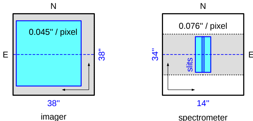
Figure 15: Field orientation and pixel scale for the imaging and spectroscopic modes of VISIR for TEL.ROT.OFFANGLE = 0° . While the imaging detector follows the normal astronomical convention, the spectroscopic detector is reversed in x -direction so that East is to the right. The gray area marks the region of the detector which is typically read-out, the spectroscopy detector being windowed in y -direction. The magenta areas mark the areas illuminated by the sky – in case of the spectrometer for the very wide slit (“OPEN”). The sizes of these usable areas on sky are given in blue (see also § 4.4).
