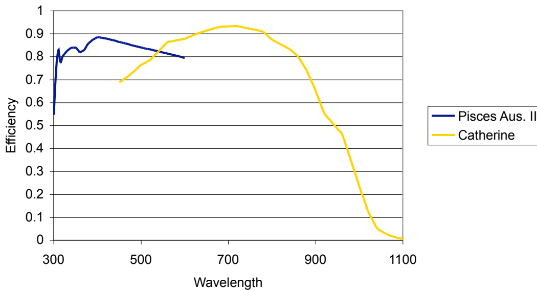
Figure 8: UVB/VIS detector efficiency.
