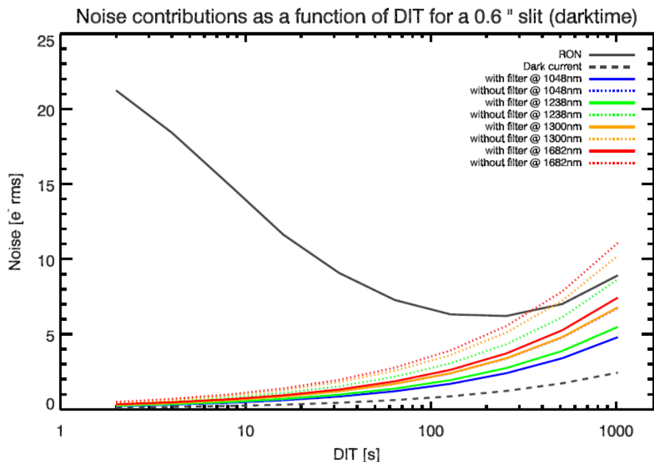
Figure 14: Noise contributions as a function of DIT for a 0.6" slit. With K-band blocking filter the background is always RON limited. Without K-band blocking filter the background is RON limited for DITs up to ~360 s at wavelength 1682 nm and 450 s at 1300nm. For longer DITs the background is sky limited.
