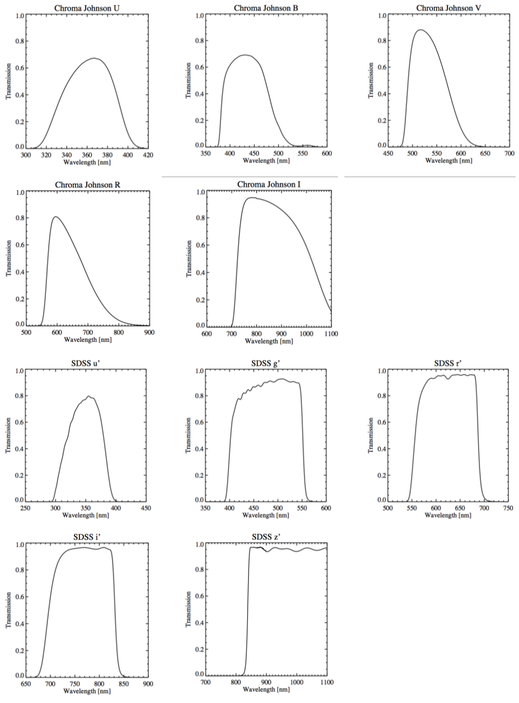
Figure 27: A&G camera filter curves.
