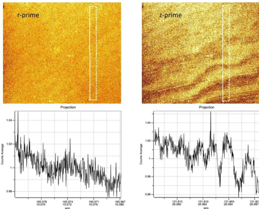
Figure 30: Fringing in r\_prime and z\_prime . The most affected filters are r\_prime , i\_prime , z\_prime , and i . The peak-to-peak amplitudes range from 2% in r\_prime to 4% in z\_prime .
