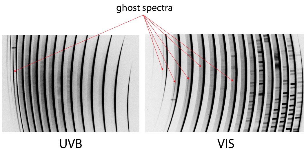
Figure 18: Ghost spectra in UVB and VIS produced by back reflection in the two dichroics.
