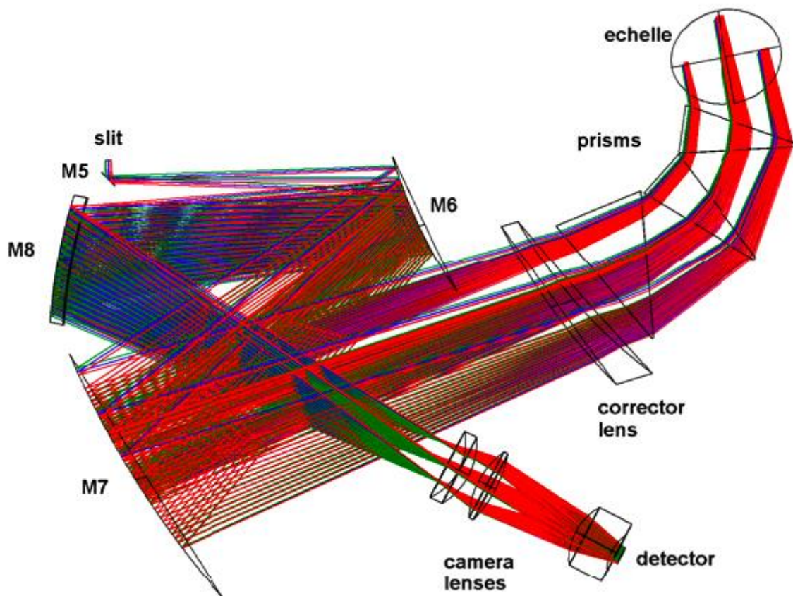
Figure 9: The NIR spectrograph optical layout.
