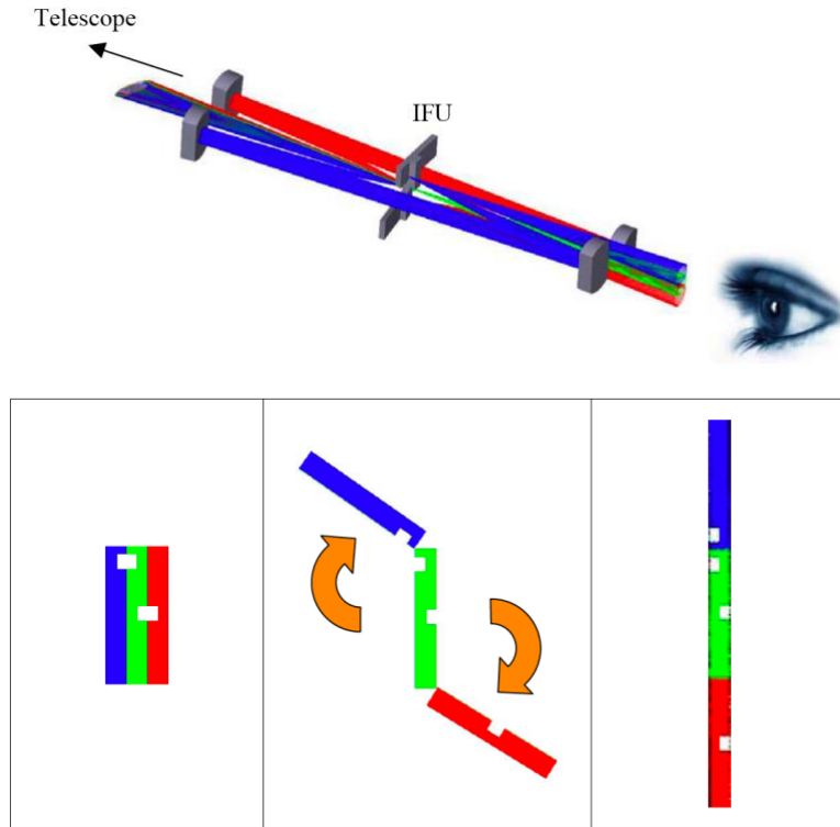
Figure 4: X-shooter IFU. The central field is directly transmitted to form the central slitlet (green), while each lateral field (blue and red) is reflected toward a pair of spherical mirrors and realigned at the end of the central slice to form the exit slit. The IFU acts such that the lateral fields seem to rotate around a corner of their small edge. The white slots are guides to help visualize the top and the bottom of each slice in the drawing.
