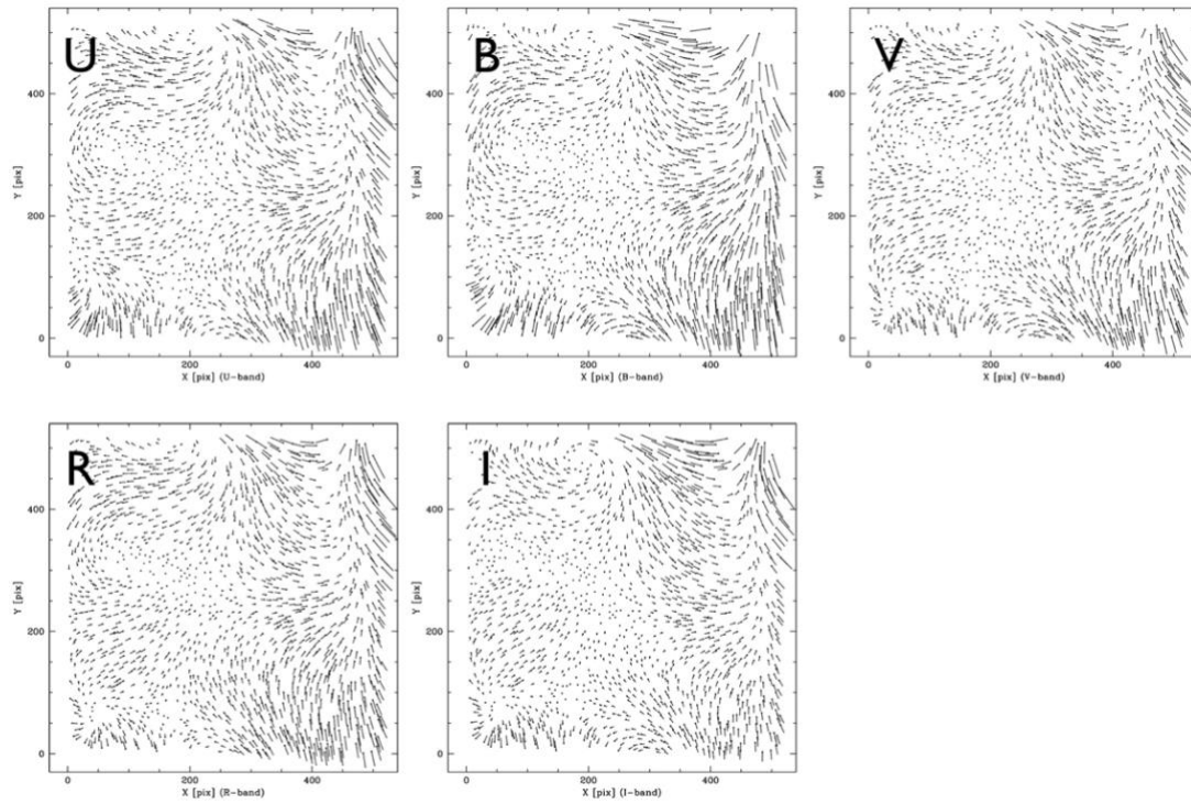
Figure 29: UBVRI distortion maps magnified x20. The difference between 2MASS and the A&G TCCD astrometry is \pm 0.1'' .
