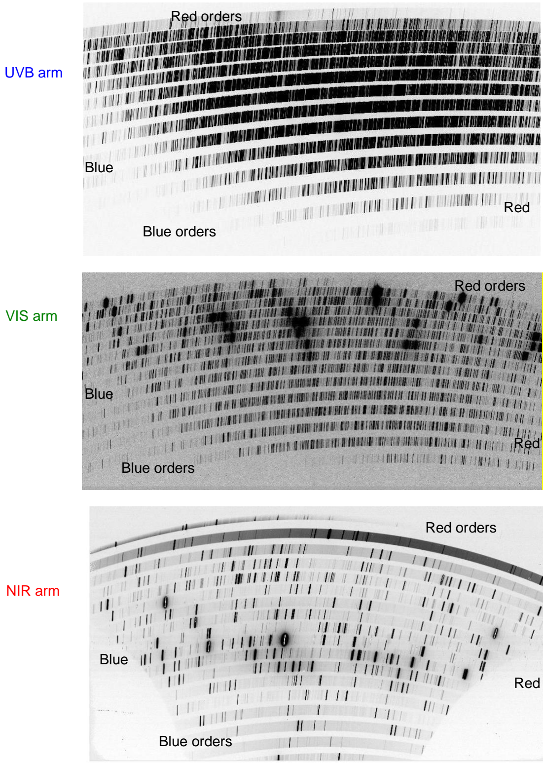
Figure 17: Example of UVB (top), VIS (middle), and NIR (bottom) calibration frames. Strong order curvature and varying slit tilt and scale are clearly visible. Note the higher thermal background at longer wavelengths for the NIR arm, in particular in the 11th order (K band).
