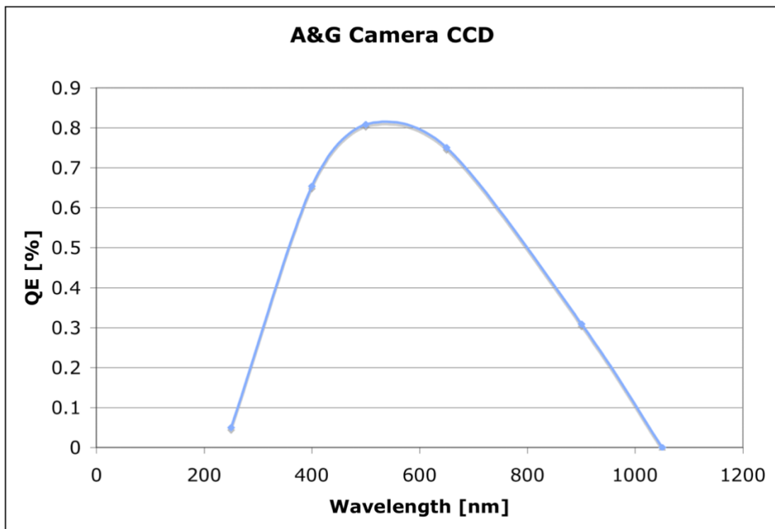
Figure 26: A&G TCCD quantum efficiency curve.
