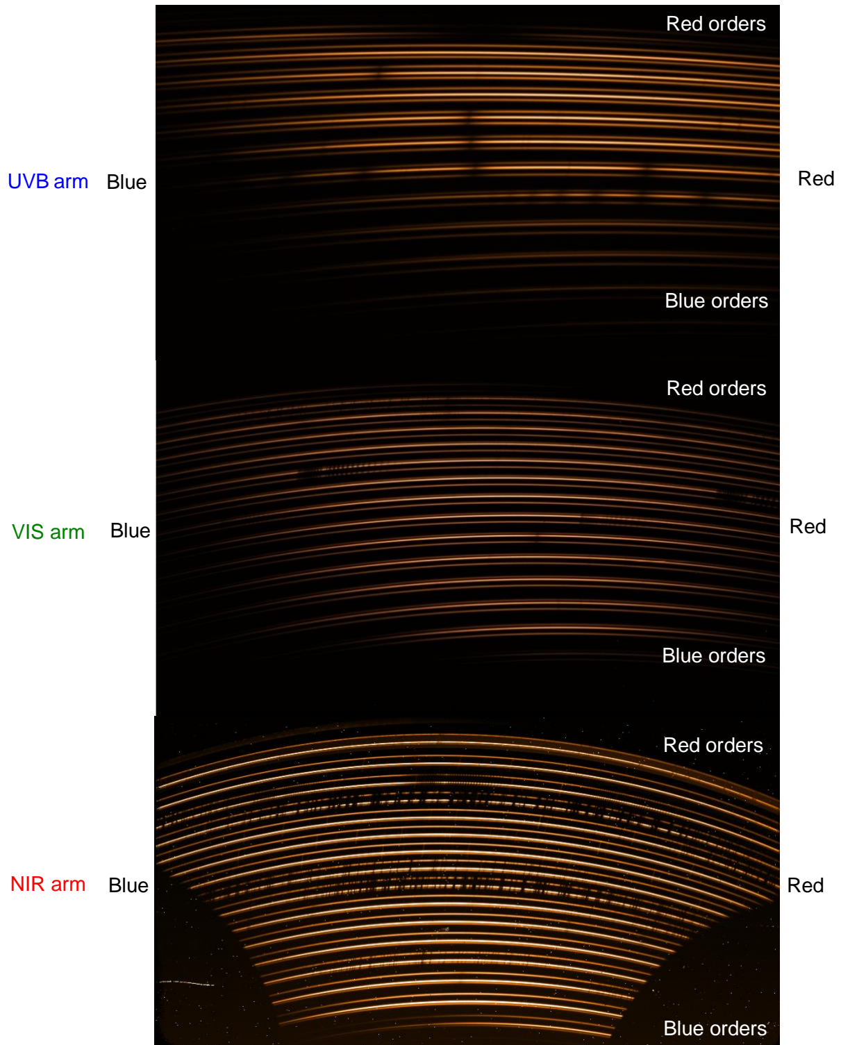
Figure 5: IFU observation showing the three slices in each order. The telluric absorption lines are visible in the VIS and NIR. The effect of the atmospheric dispersion is also observed (change of distance between the slices between blue and red orders in the UVB/VIS arms).
