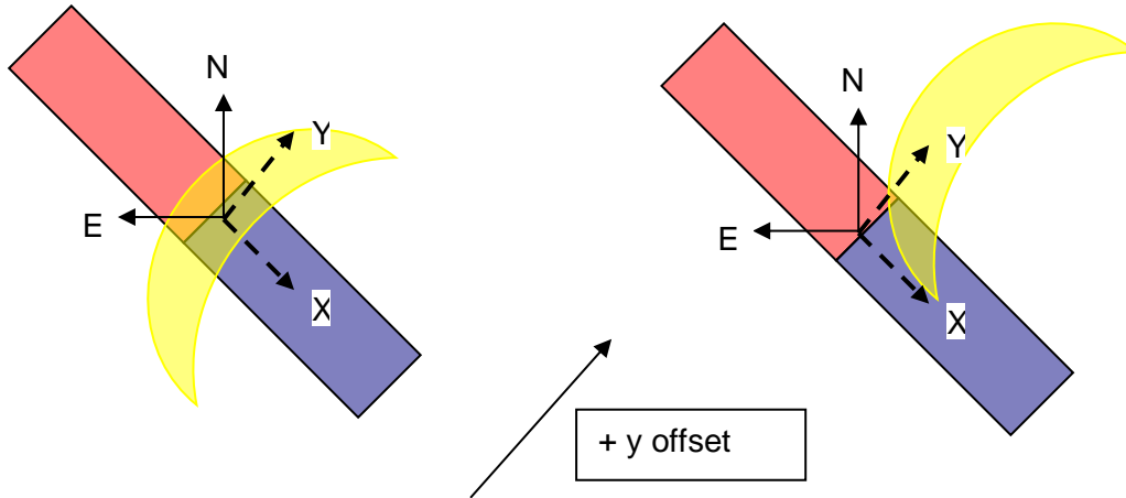
Figure 35: The offset with PA= +45 degrees shows a positive offset in y axis. The object moves in +y, while the slit moves in the -y axis.
