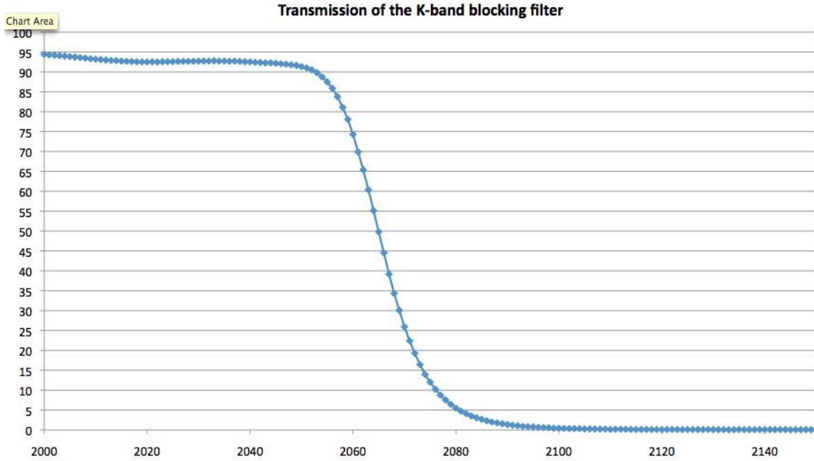
Figure 10: Transmission curve of the K-band blocking filter.
