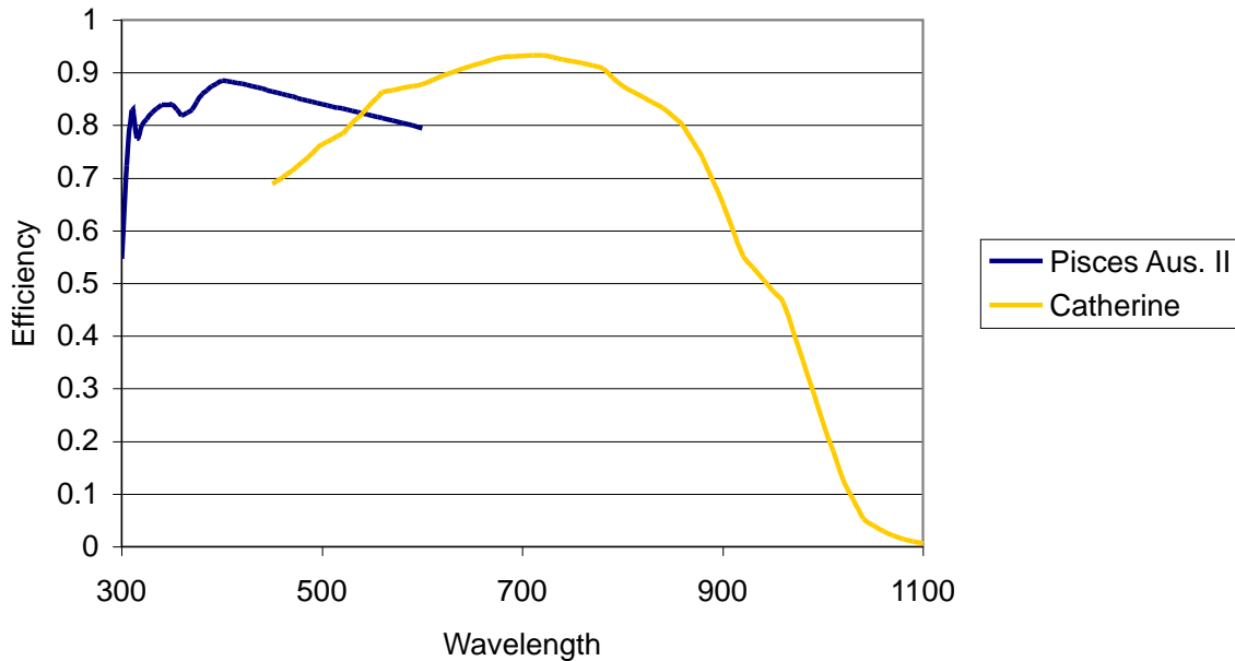
Figure 8: UVB/VIS detector efficiency.
