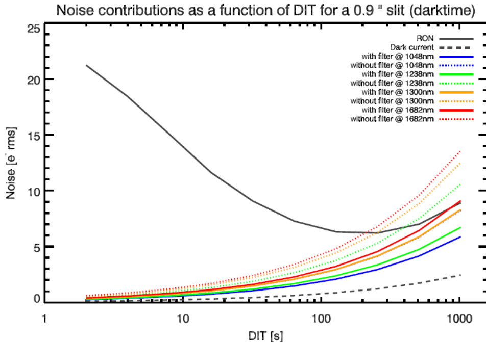
Figure 13: Noise contributions as a function of DIT for the 0.9" slit. With the K-band blocking filter the background is always RON limited for DITs shorter than 1000 s, independent on the wavelength. For DITs longer than 1000 s, the background is sky limited above 1682 nm. Without the K-band blocking filter the background is RON limited for DIT up to 200 s to 300 s at wavelengths 1682 nm and 1300 nm. For longer DITs the background is sky limited.
