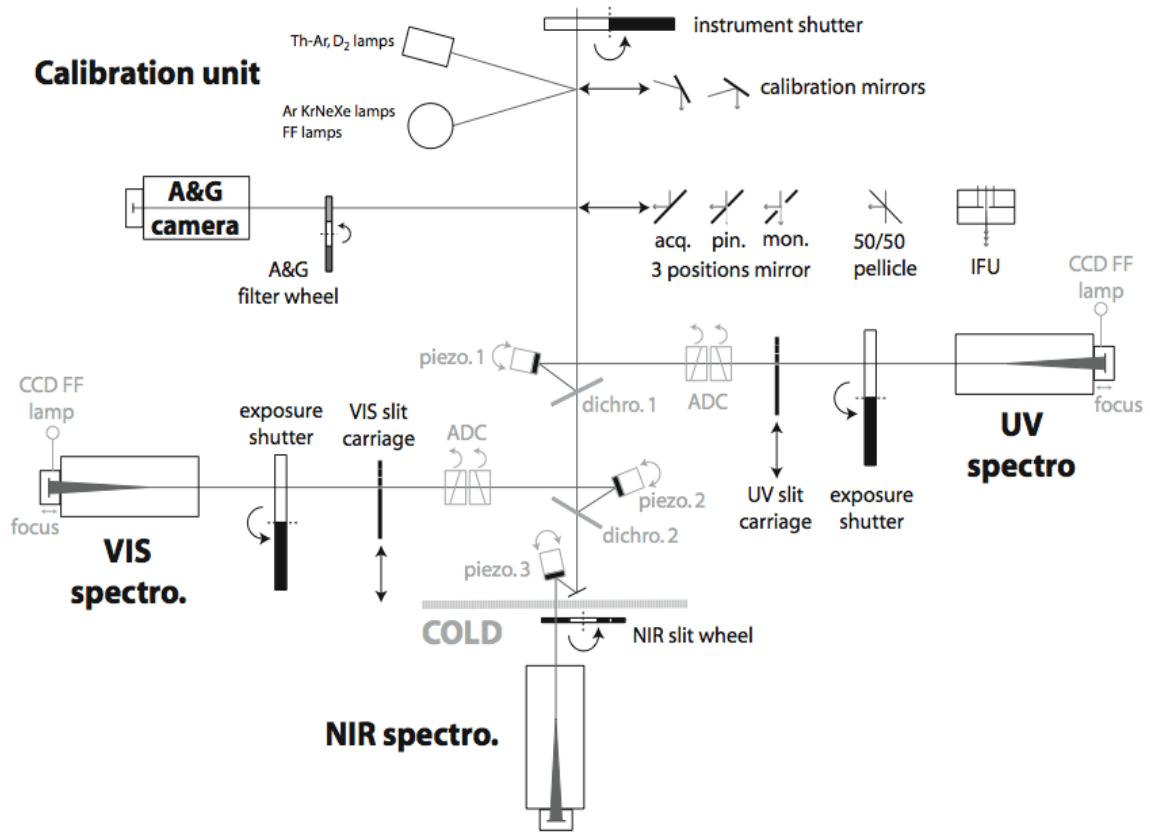
Figure 2: Schematic overview of the opto-mechanical design of X-shooter.
