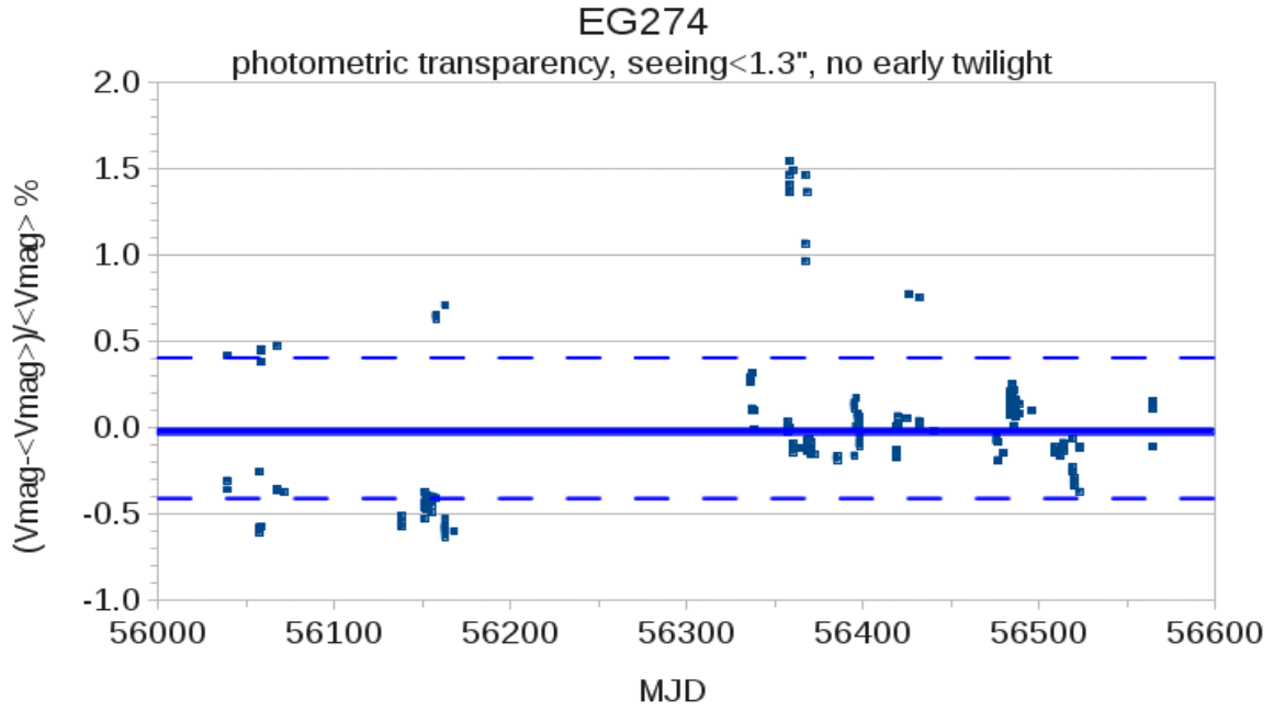
Figure 28: Photometric transparency.
