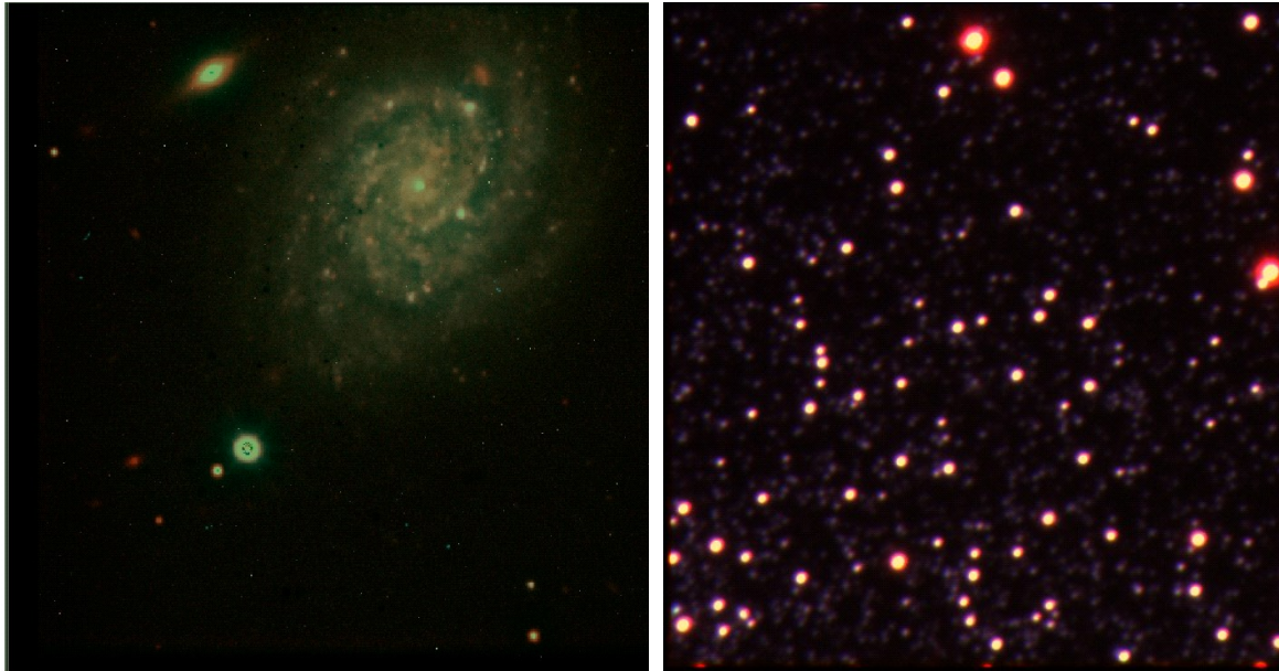
Figure 25: Three color (BVI) image of a galaxy with a supernova (left) and of a small field of 47Tuc (right).
