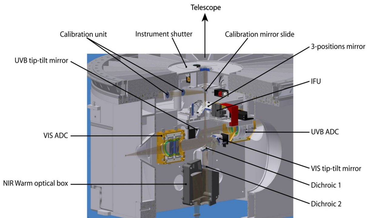
Figure 3: 3D view of a cut through the backbone.
