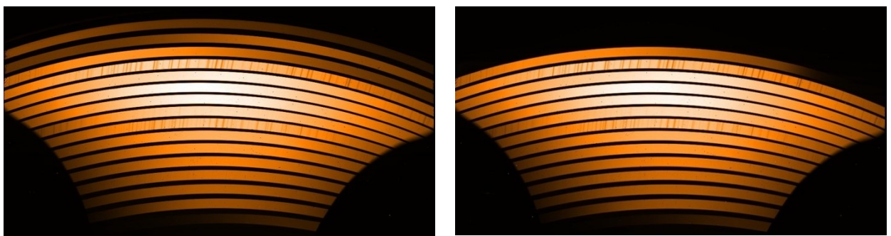
Figure 11: Flatfield frames for the normal 0.9" NIR slit (left) and for the 0.9" with K-band blocking filter (right). The last orders are cut with the K-band blocking filter.
