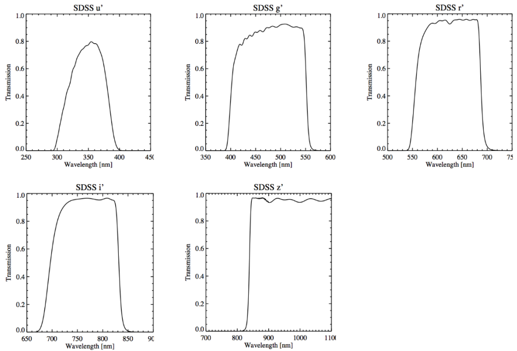
Figure 27: A&G camera filter curves.
