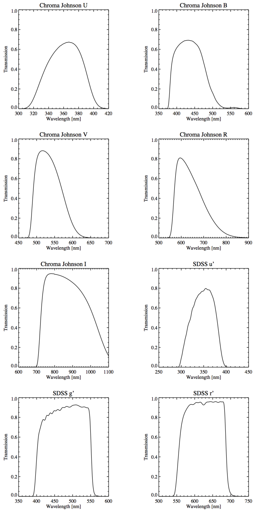
Figure 3: A&amp;G camera filter curves.
