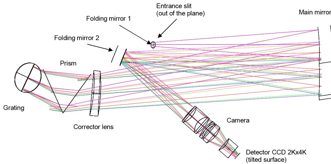
Figure 7: The UVB spectrograph optical layout
