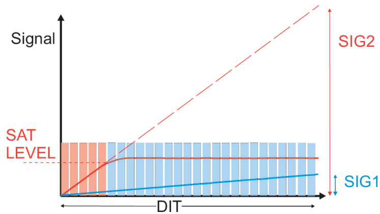
Figure 9: Saturation threshold for nondestructive sampling and extrapolation of detector signal for high flux levels. For pixels with high flux (red) only readout values below SATLEVEL (orange rectangles) are taken into account in the calculation of the slope and values written in the FITS files are extrapolated to the full DIT (SIG2). For low flux pixels (blue) all nondestructive readouts are used (light blue rectangles). Figure courtesy of Finger et al. (2008).
