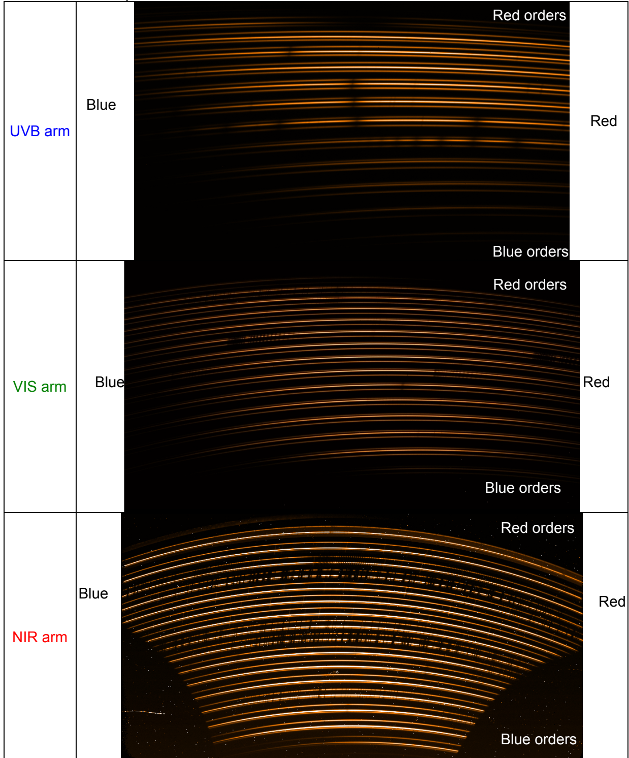
Figure 5: IFU telluric standard star (B-type star). One can note the three slices in each order of each arm. The telluric absorption lines are easily visible in the VIS and NIR arms.
