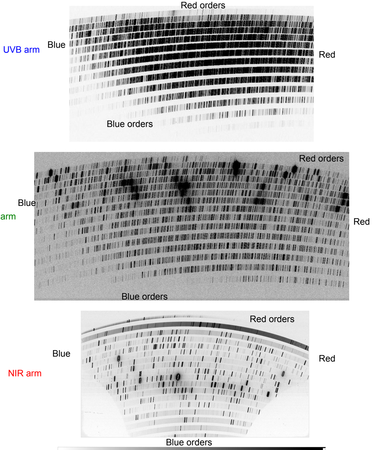
Figure 10: example of UVB (top), VIS (middle) and NIR (bottom) calibration frames. Strong order curvature and varying slit tilt and scale are clearly visible. Note for the NIR arm the higher thermal background in longer wavelength. This is specially the case in the 11 th order that corresponds to the K band.
