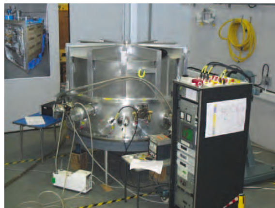
Figure 3 (right). The KMOS main cryostat undergoing its first cooldown cycles. The closed-cycle coolers are visible around the base of the cryostat; the remaining ports contain the feedthroughs for some of the 1500 electrical connections into the cryostat. The electronics rack to the right contains all the housekeeping electronics and will eventually be mounted on the Nasmyth platform.
